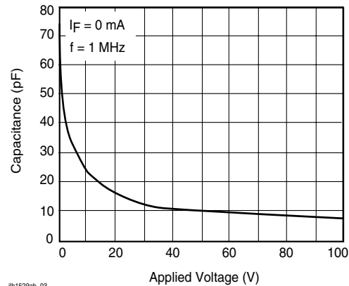
Figure 4. Switch Capacitance vs. Applied Voltage
