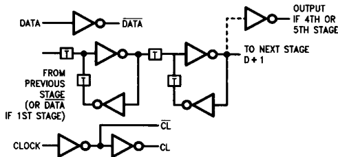
TL/F/5942-1
