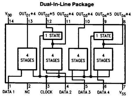
TL/F/5942-2
