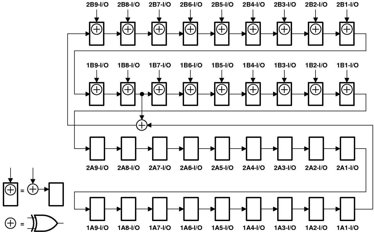
Figure 8. 36-Bit PSA Configuration ( 1\overline{0EAB} = 2\overline{0EAB} = 1 , 1\overline{0EBA} = 2\overline{0EBA} = 0 )
