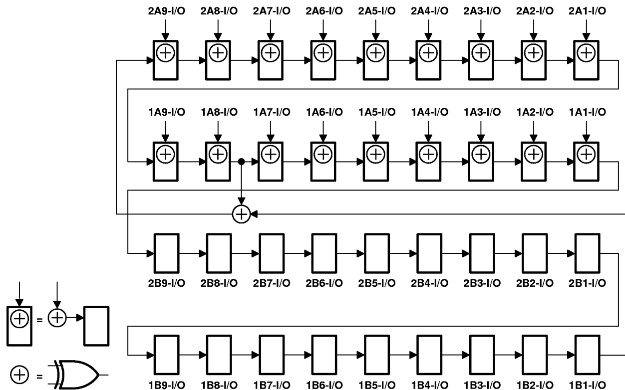
Figure 7. 36-Bit PSA Configuration ( 1\overline{0EAB} = 2\overline{0EAB} = 0, 1\overline{0EBA} = 2\overline{0EBA} = 1 )
