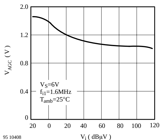
Figure 12. AM section: AGC voltage (at Pin 22)
