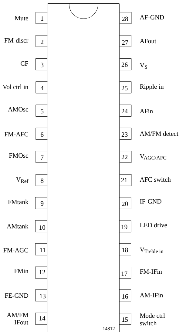
Figure 2. Pinning
