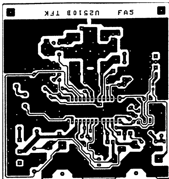
Figure 19. PC-board
