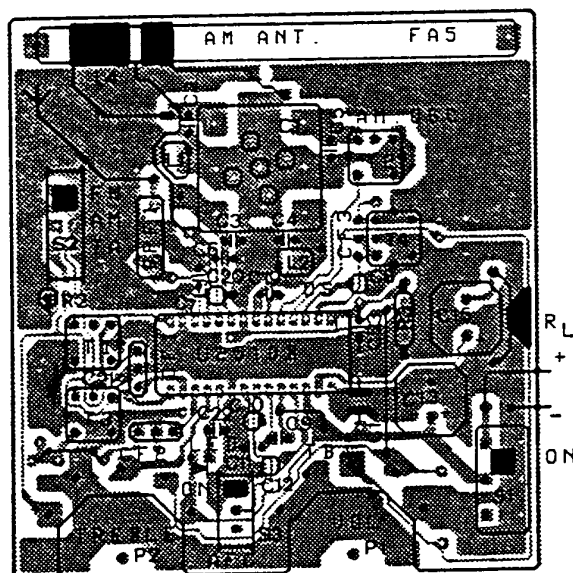
Figure 19. PC-board
