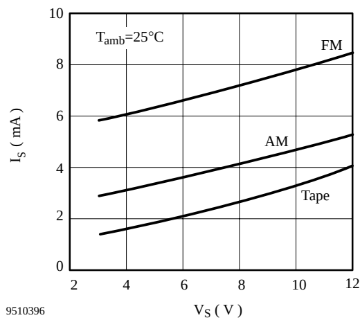
Figure 3. Quiescent current
