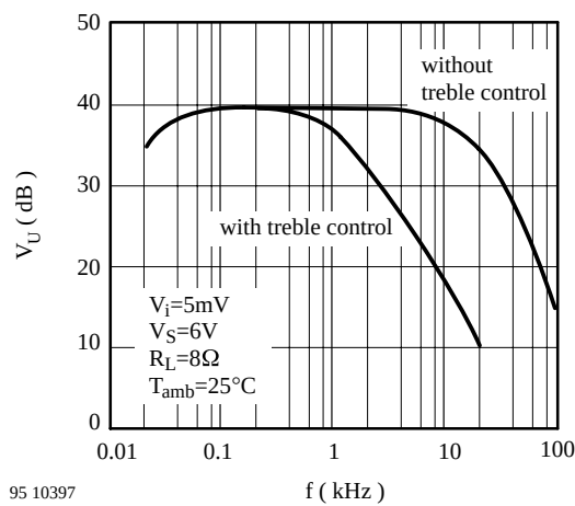
Figure 4. AF section
