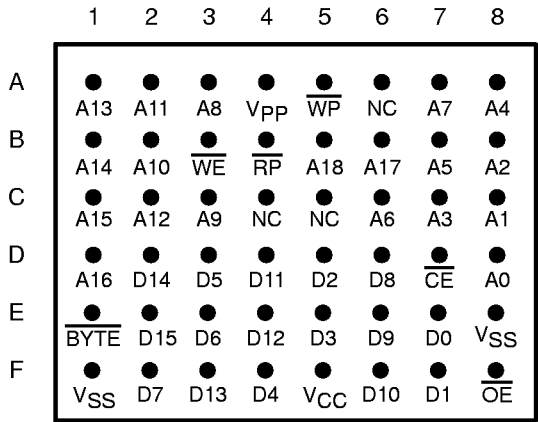
TMS28F800Axy 48-BALL µBGA (TOP VIEW)
