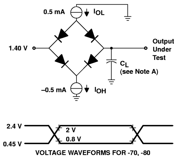
Figure 9. 3-V Testing Load Circuit and Voltage Waveform
