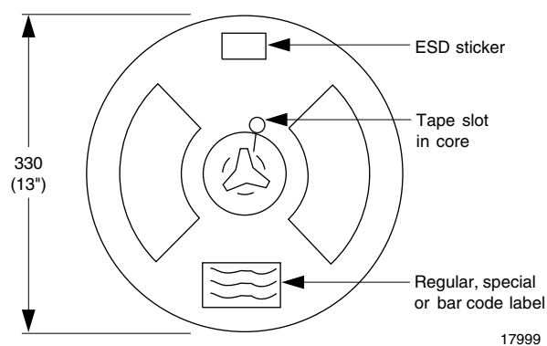
Fig. 17 - Tape and Reel Shipping Medium
