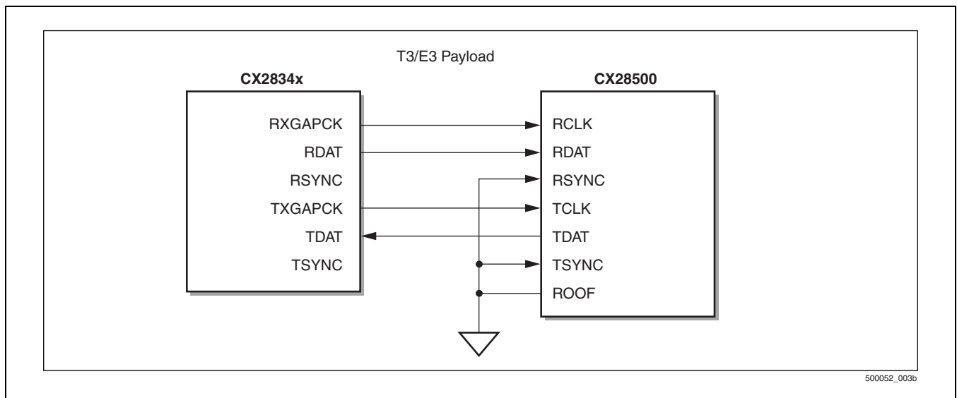
Figure C-3. T3/E3 Framer Connection with HDLC Controller (T3/E3 Payload Path)
