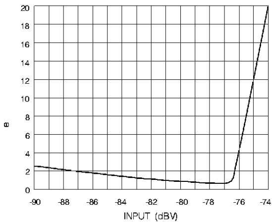
Fig. 9 THD vs Input (Blocks A to E)
