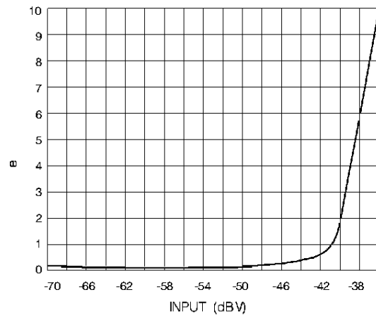
Fig.10 THD vs Input (Telecoil)
