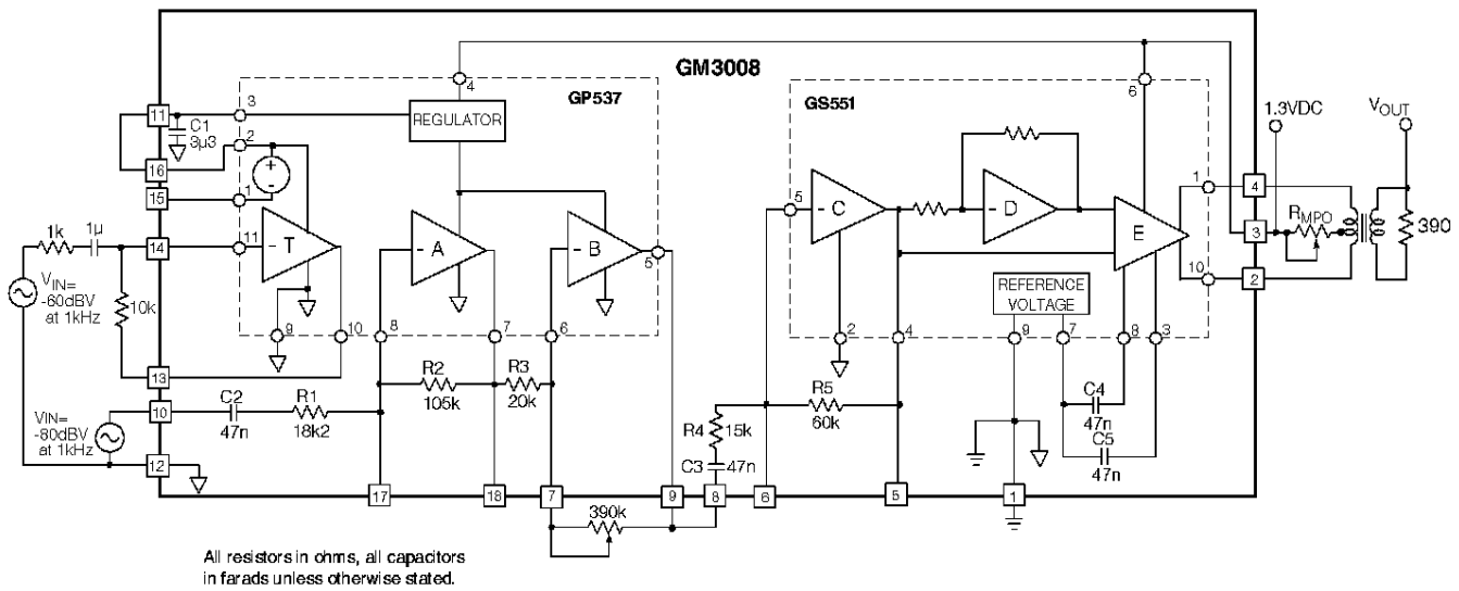
Fig. 4 Characterization Circuit (used to generate Typical Curves)
