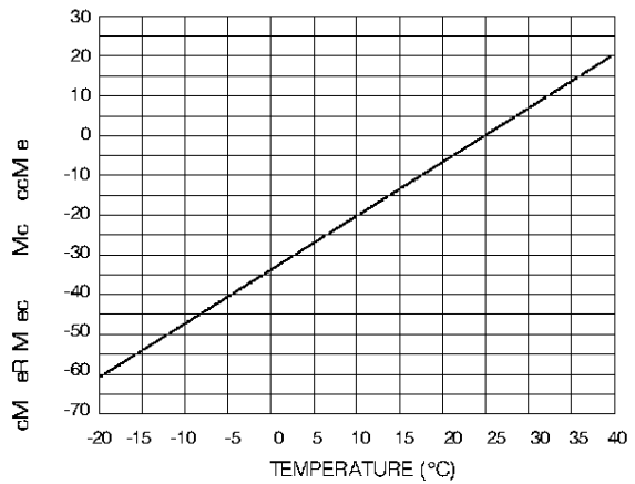
Fig. 16 Transducer Current vs Temperature
