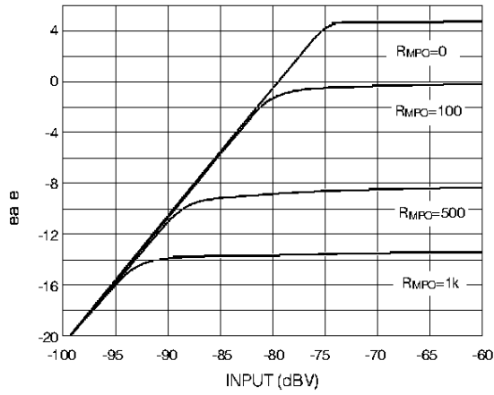
Fig. 11 Maximum Power Output vs R_{MPO}
