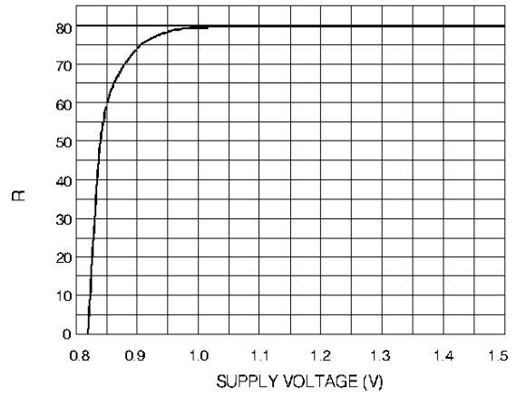
Fig. 12 Gain vs Supply Voltage
