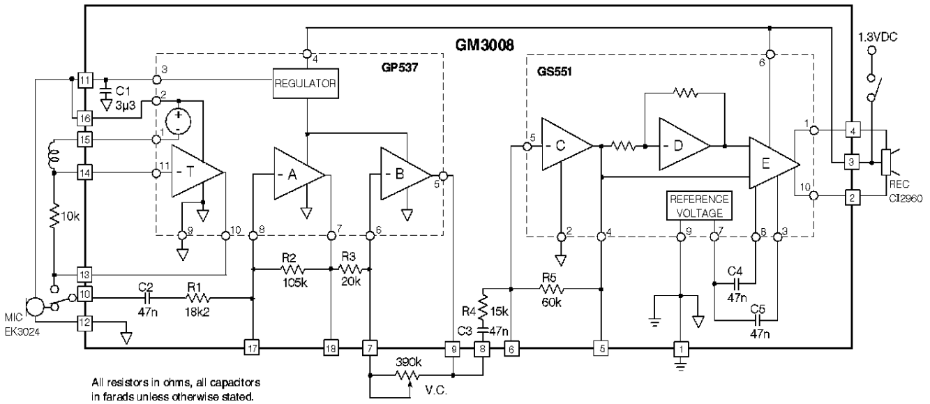
Fig. 2 Typical Hearing Instrument Application
