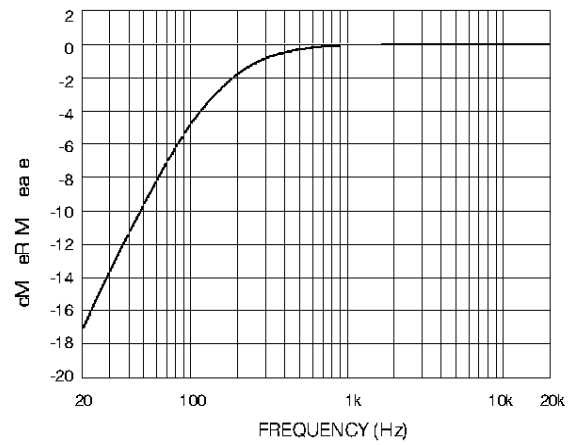
Fig. 8 Frequency Response (Telecoil)
