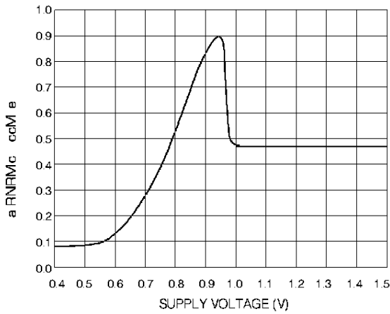
Fig. 13 Amplifier Current vs Supply Voltage
