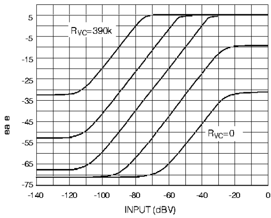
Fig. 5 Input vs Output as R_{VC} is Varied (Blocks A to E)
