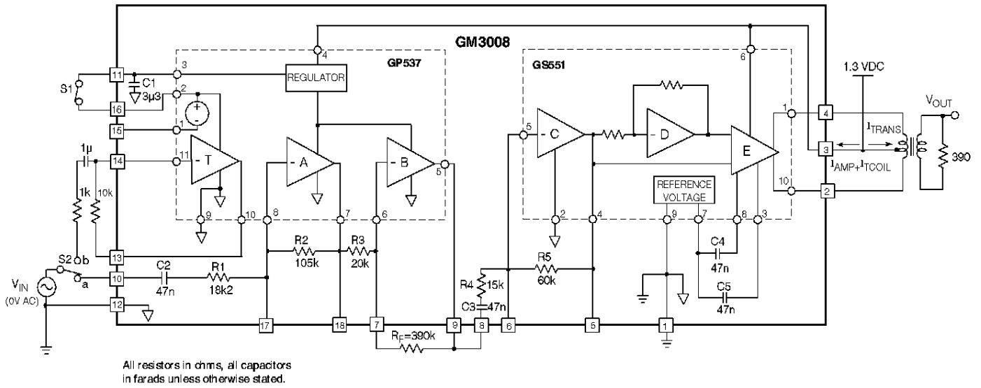
Fig. 1 Production Test Circuit
