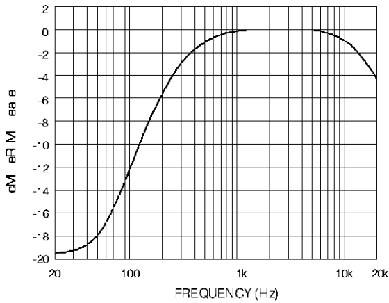
Fig. 7 Frequency Response (Blocks A to E)
