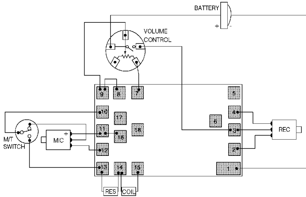
Fig. 3 Maximum Components Configuration Assembly Diagram of GM3008
