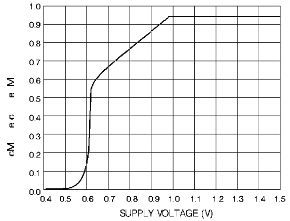
Fig. 14 Regulator Voltage vs Supply Voltage
