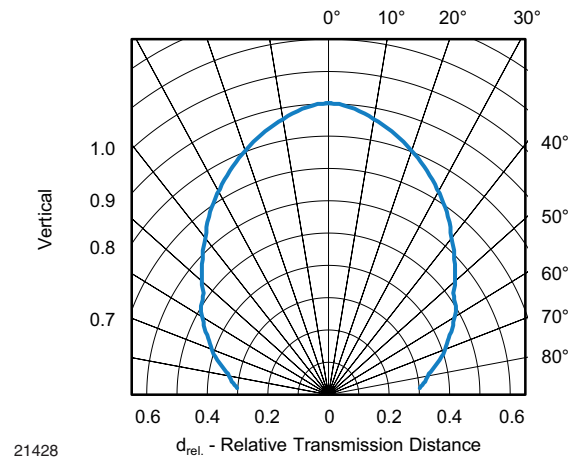
Fig. 5 - Vertical Directivity
