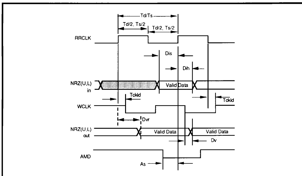
FIGURE 7: Disk Interface Timing
