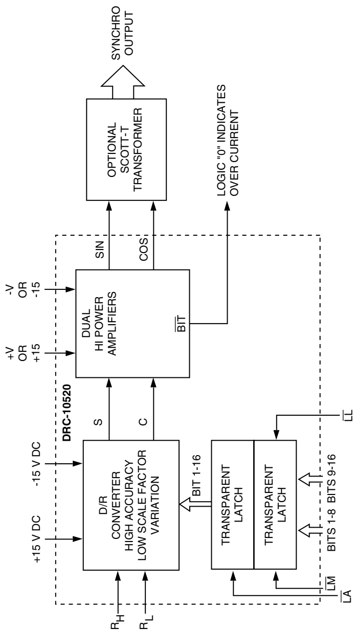
FIGURE 1. DRC-10520 BLOCK DIAGRAM
