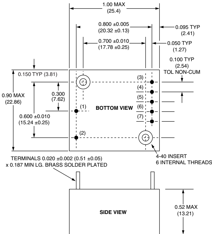
FIGURE 4. POWER TRANSFORMER (29306, 33920) MECHANICAL OUTLINE
