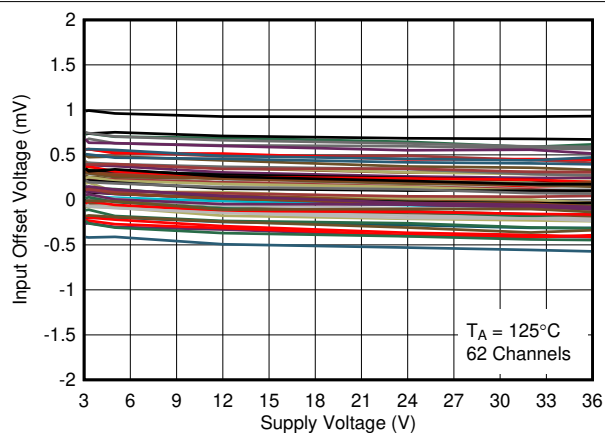
Figure 7-14. Input Offset Voltage vs. Supply Voltage at 125^\circ\text{C}
