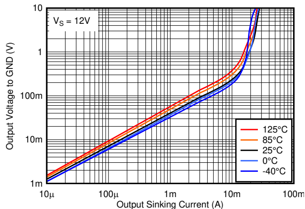
Figure 7-21. Output Low Voltage vs. Output Sinking Current at 12V
