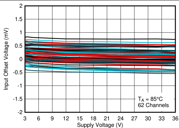
Figure 7-13. Input Offset Voltage vs. Supply Voltage at 85^\circ\text{C}
