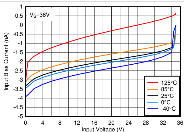
Figure 7-18. Input Bias Current vs. Input Voltage at 36\text{ V}
