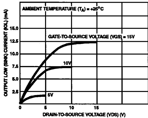
FIGURE 4. MINIMUM N-CHANNEL OUTPUT LOW (SINK) CURRENT CHARACTERISTICS
