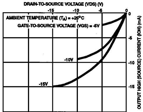
FIGURE 6. MINIMUM P-CHANNEL OUTPUT HIGH (SOURCE) CURRENT CHARACTERISTICS
