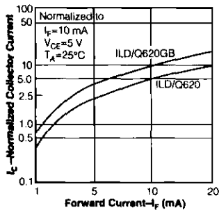
Figure 9. Collector current versus diode forward current
