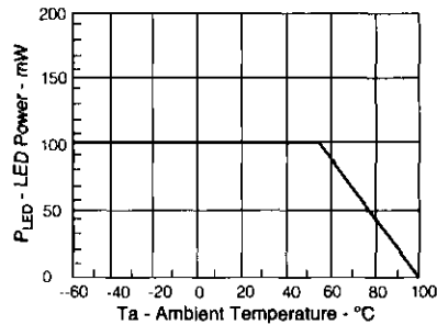
Figure 8. Maximum LED power dissipation
