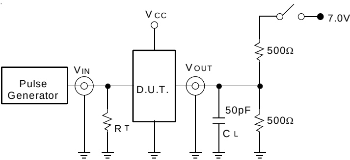
AC Test Circuit
