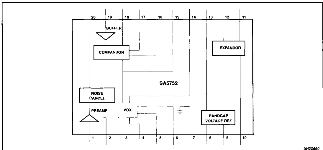
Figure 2. Block Diagram
