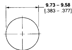
Recommended Panel Cutout for 1274032-1
