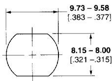
Recommended Panel Cutout for 415332-1 and 415888-1
