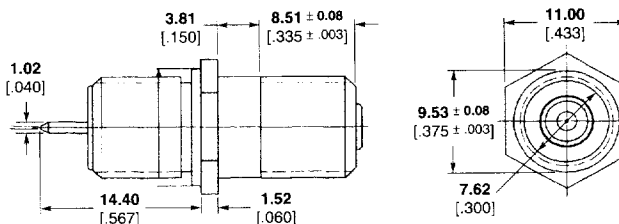
Part No. 1274064-1
