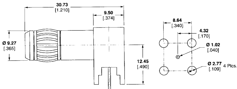
Part No. 1274401-1
