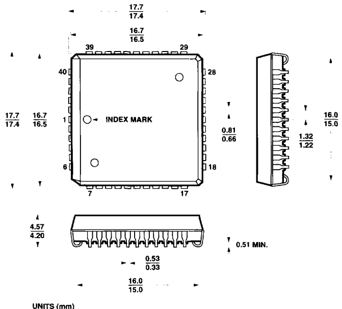
Figure 8. HBCR-2211 Mechanical Specifications.
