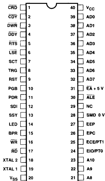
Figure 5. HBCR-2210 Parallel Pinout.
