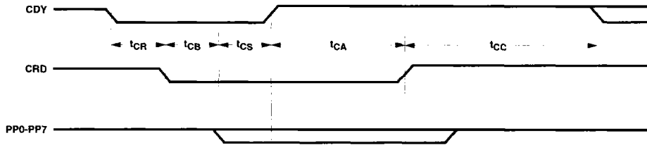
Figure 1. Host Commands Received by Decode IC (Reader).
