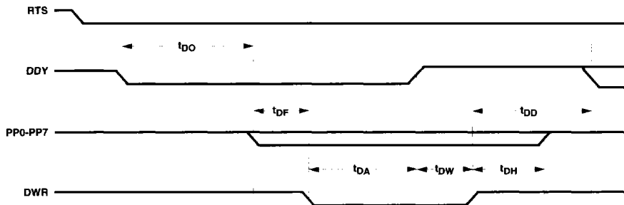
Figure 2. Decoder IC Data Sent to Host.
