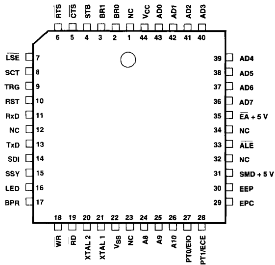
Figure 4. HBCR-2211 Serial Pinout.
