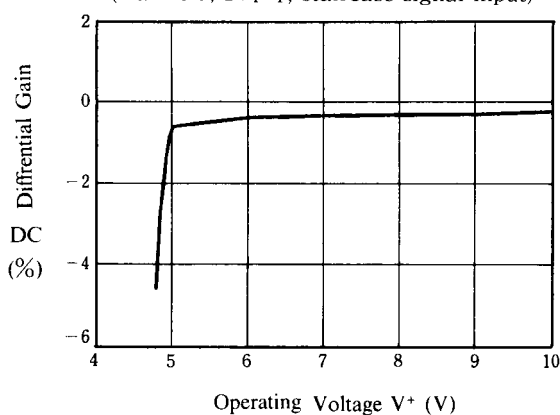
Differential Gain vs. Operating Voltage
