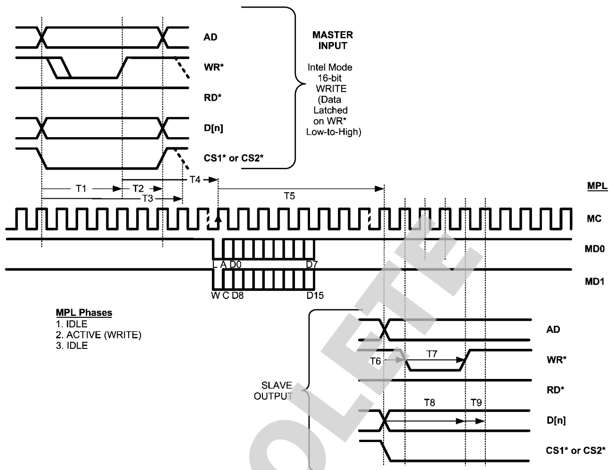
FIGURE 11. WRITE — i80 CPU Interface
