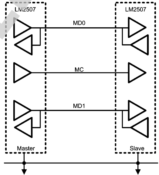
FIGURE 3. MPL Point-to-Point Bus
