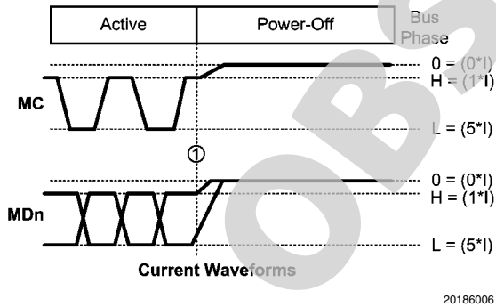
FIGURE 7. Bus Power Down Timing
