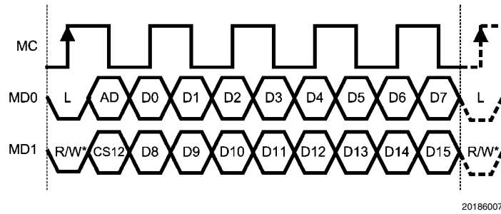
FIGURE 8. 16-bit CPU WRITE Transaction
