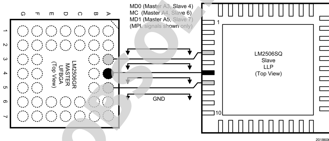
FIGURE 18. MPL Interface Layout – microArray to LLP Package
