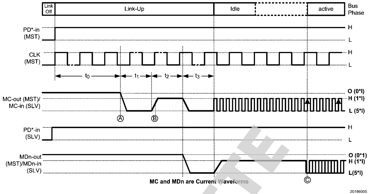
FIGURE 6. Bus Power Up Timing
