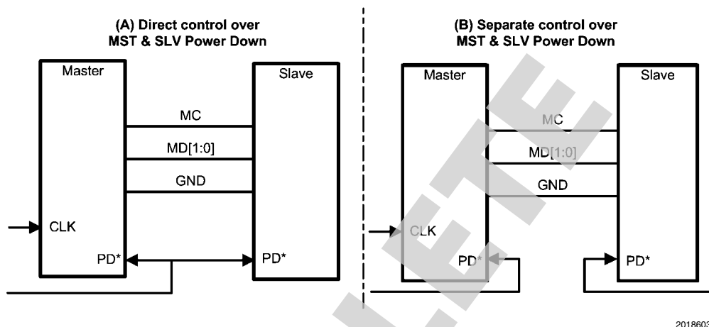
FIGURE 15. Power Down Control Options
