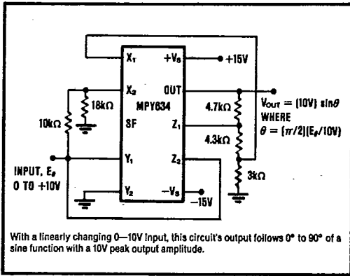
FIGURE 8. Sine-Function Generator.
