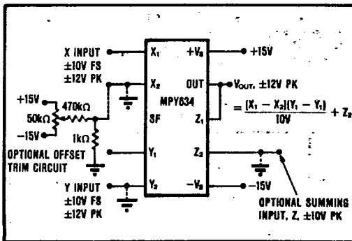
FIGURE 2. Basic Multiplier Connection.
