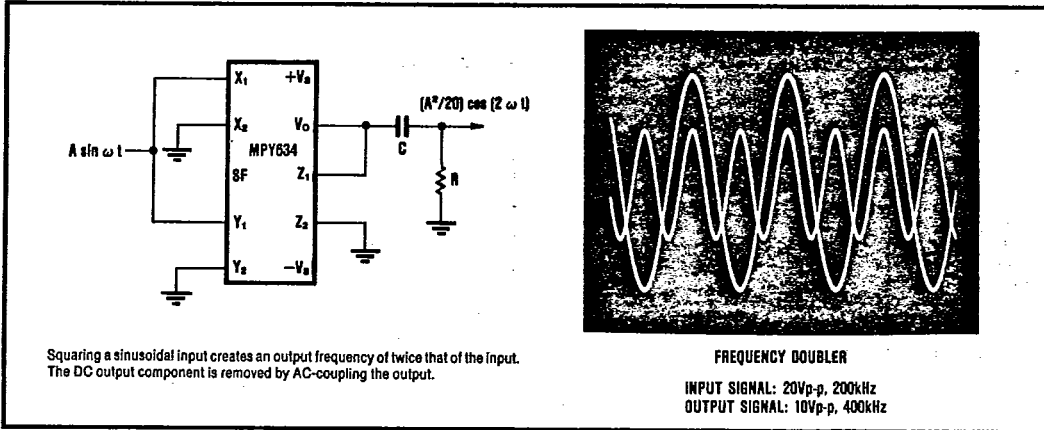
FIGURE 10. Frequency Doubler.
