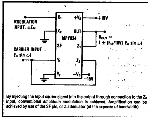
FIGURE 9. Linear AM Modulator.
