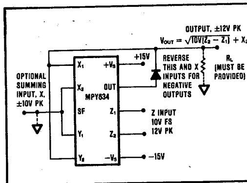
FIGURE 5. Square-Rooter Connection.
