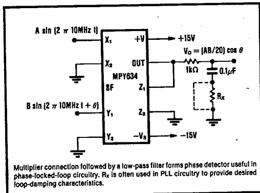
FIGURE 6. Phase Detector.
