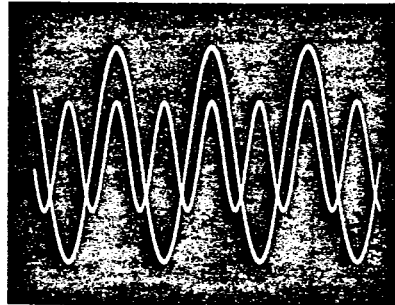
FREQUENCY DOUBLER
