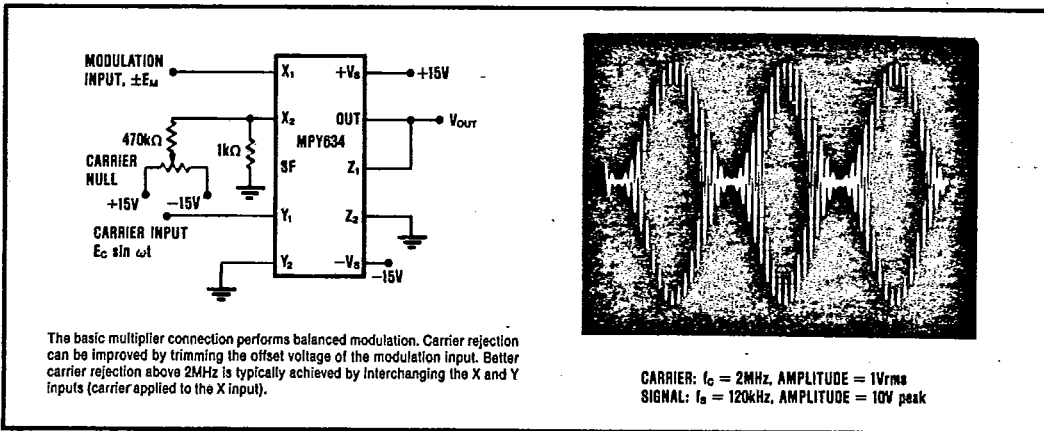
FIGURE 11. Balanced Modulator.
