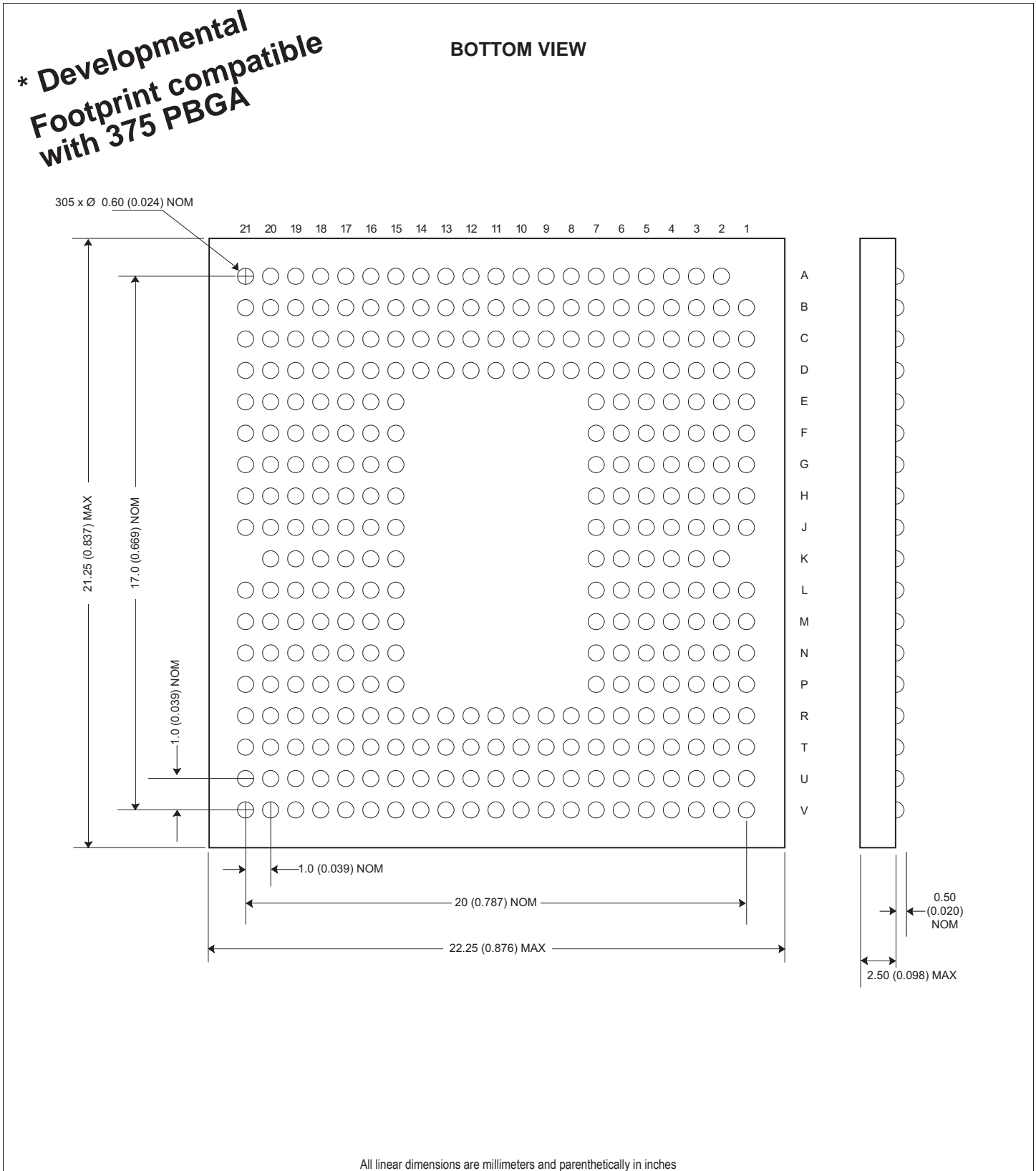
FIGURE 16A – PACKAGE DIMENSION: 305 PLASTIC BALL GRID ARRAY (PBGA) FOR W3J128M72G-XLBX*
