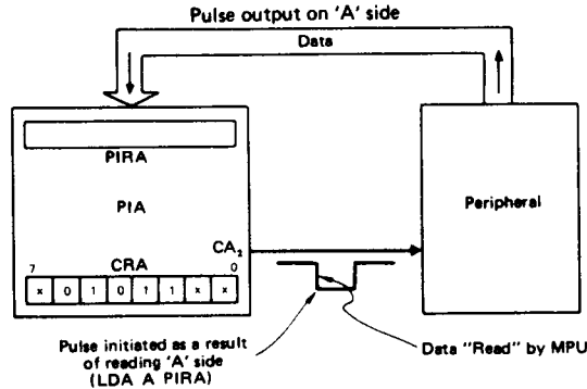
Figure 20 Bits 5, 4, 3 of CRA = 101 (Pulse Mode)
