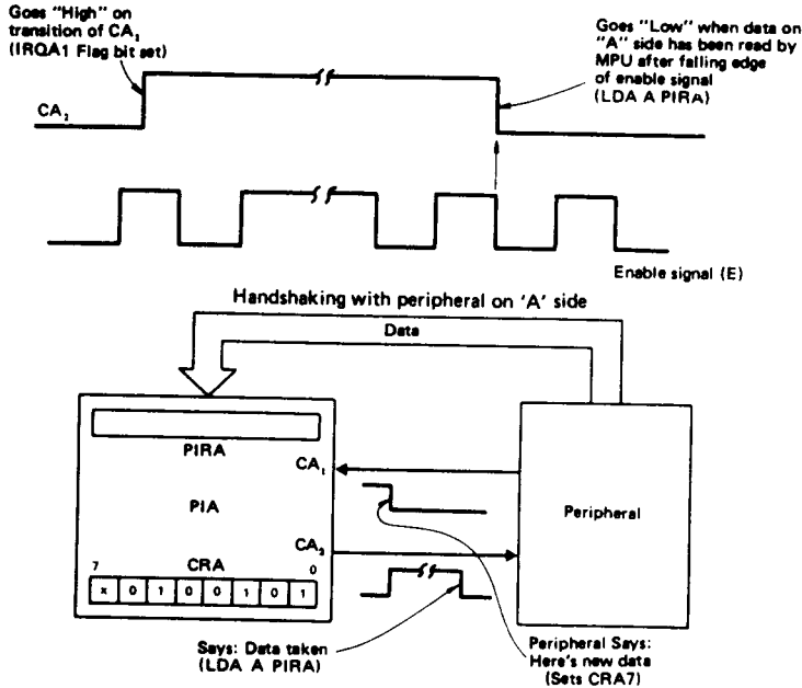
Figure 18 Bits 5, 4, 3 of CRA = 100 (Hand-shake Mode)
