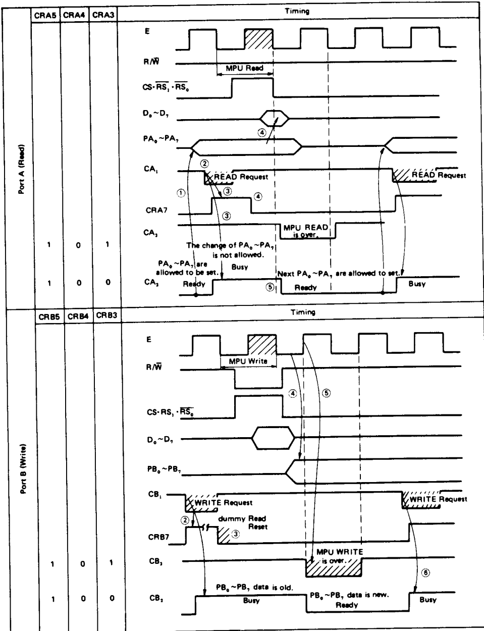
Figure 17 Timing of Hand-shake Mode and Pulse Mode
