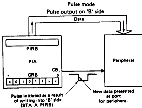
Figure 21 Bits 5, 4, 3 of CRB = 101 (Pulse Mode)
