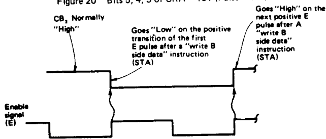
Figure 20 Bits 5, 4, 3 of CRA = 101 (Pulse Mode)
