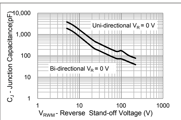
Fig.4 Typical Capacitance
