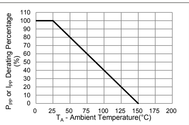
Fig.2 Derating Curve
