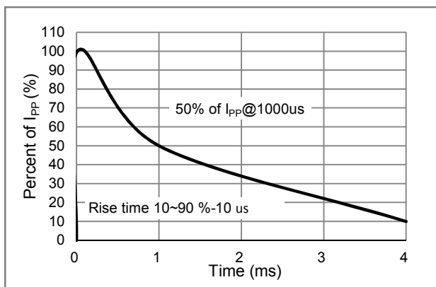
Fig.3 10/1000us Pulse Waveform
