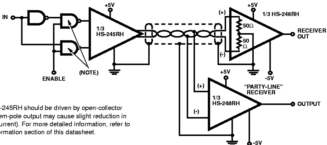
FIGURE 3. TYPICAL APPLICATION
