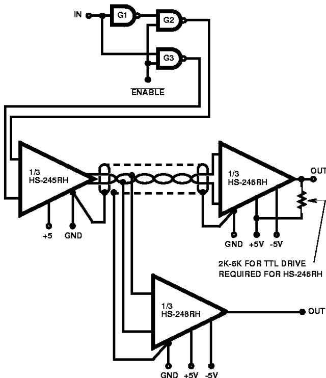
FIGURE 6. TYPICAL DATA TRANSMISSION SYSTEM
