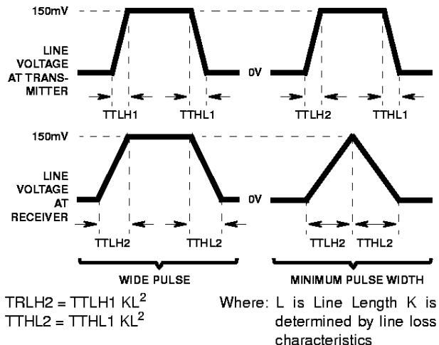
FIGURE 7. TRANSMISSION LINE WAVE-SHAPING
