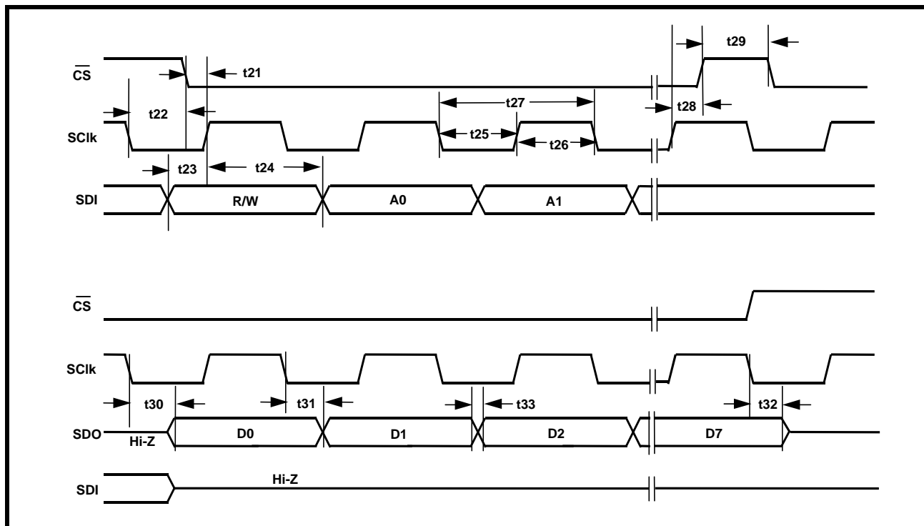
FIGURE 10. TIMING DIAGRAM FOR THE MICROPROCESSOR SERIAL INTERFACE
