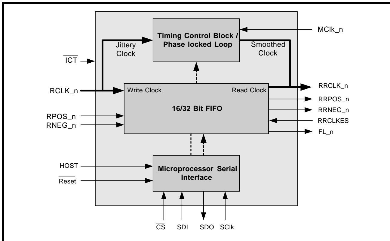
FIGURE 6. ILLUSTRATION OF OF A TYPICAL CHANNEL_N OF THE XRT71D03 (CONFIGURED TO OPERATE IN THE HOST MODE)
