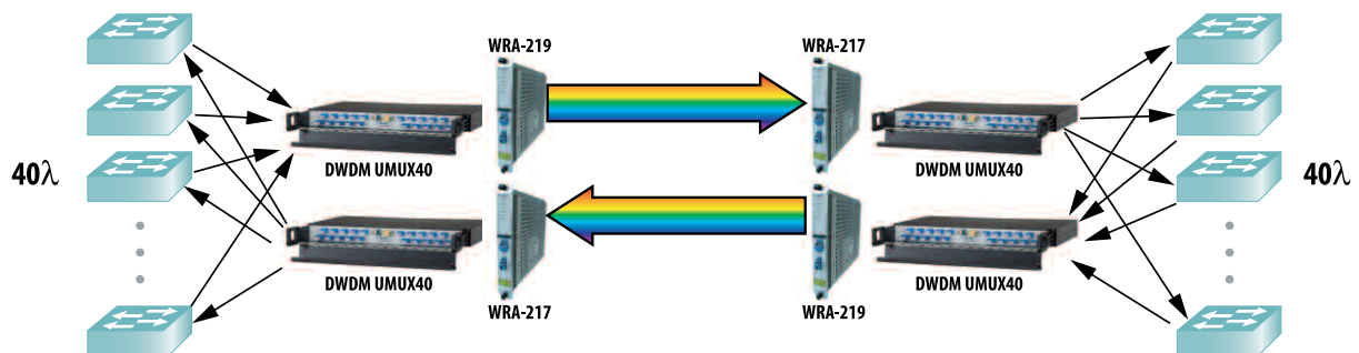
Point-to-point amplified link
