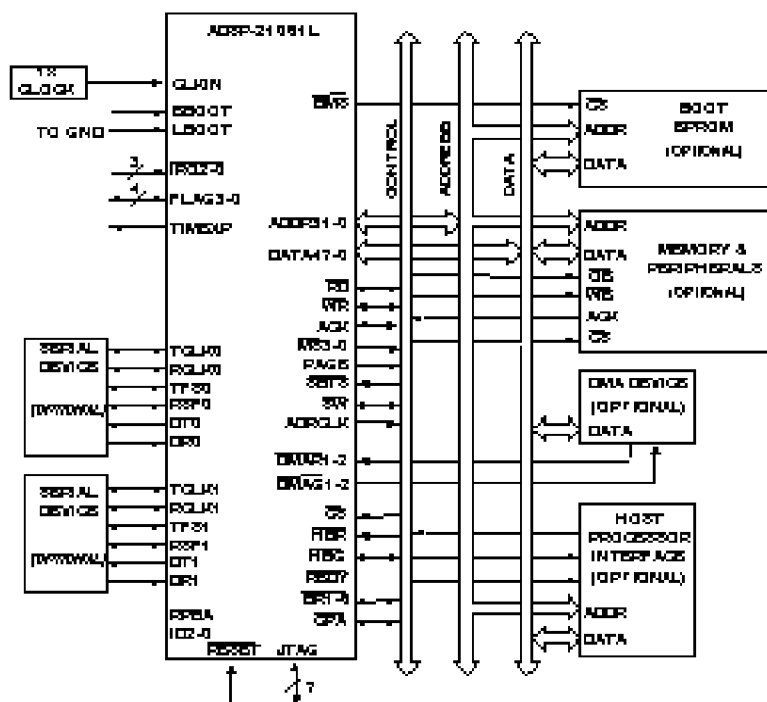
Figure 2 ADSP-21061L System
