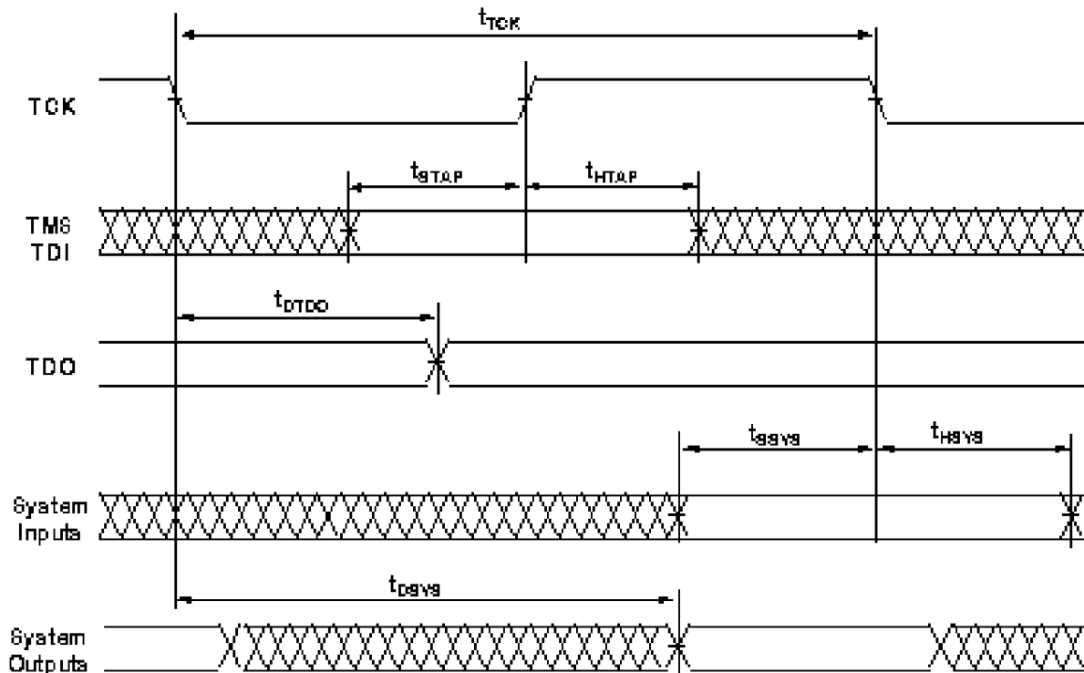
Figure 25 JTAG Test Access Port & Emulation
