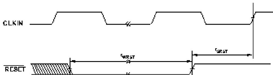
Figure 9 Reset
