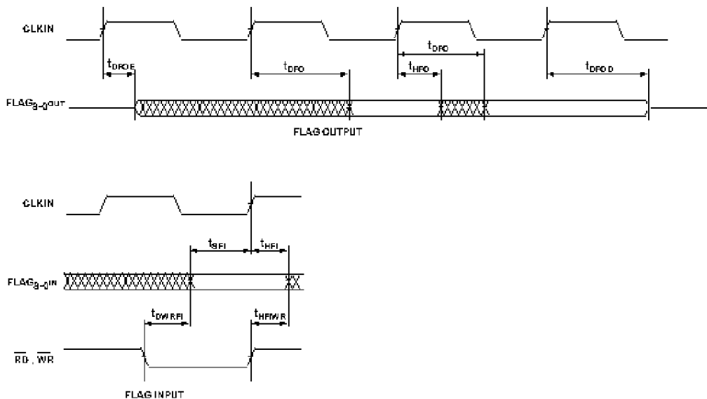
Figure 12 Flags
