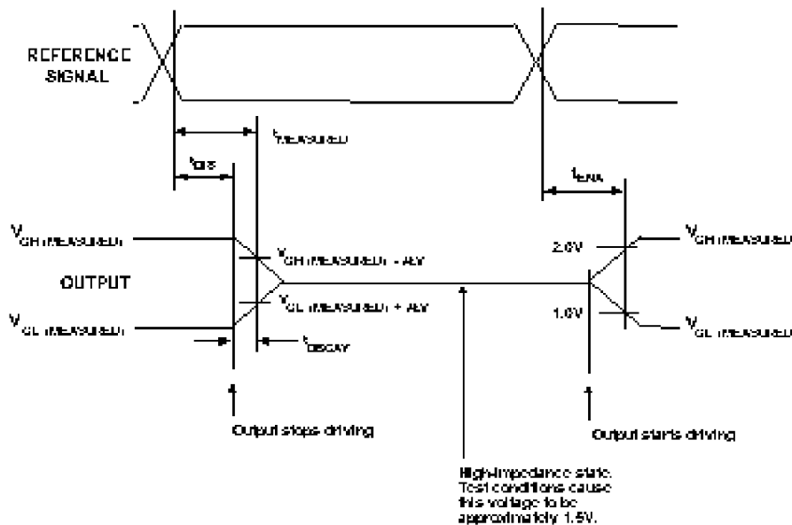
Figure 27 Output Enable
