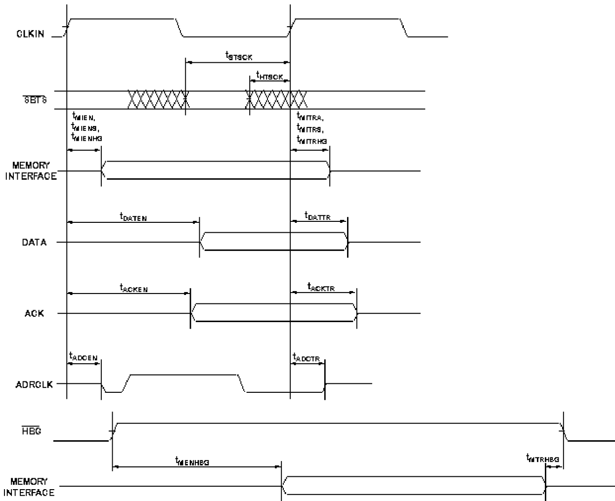
Figure 20 Three-State Timing
