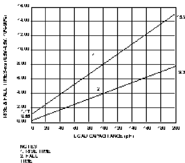
Figure 30 Typical Rise Time (10%-90% V DD ) vs. Load Capacitance
