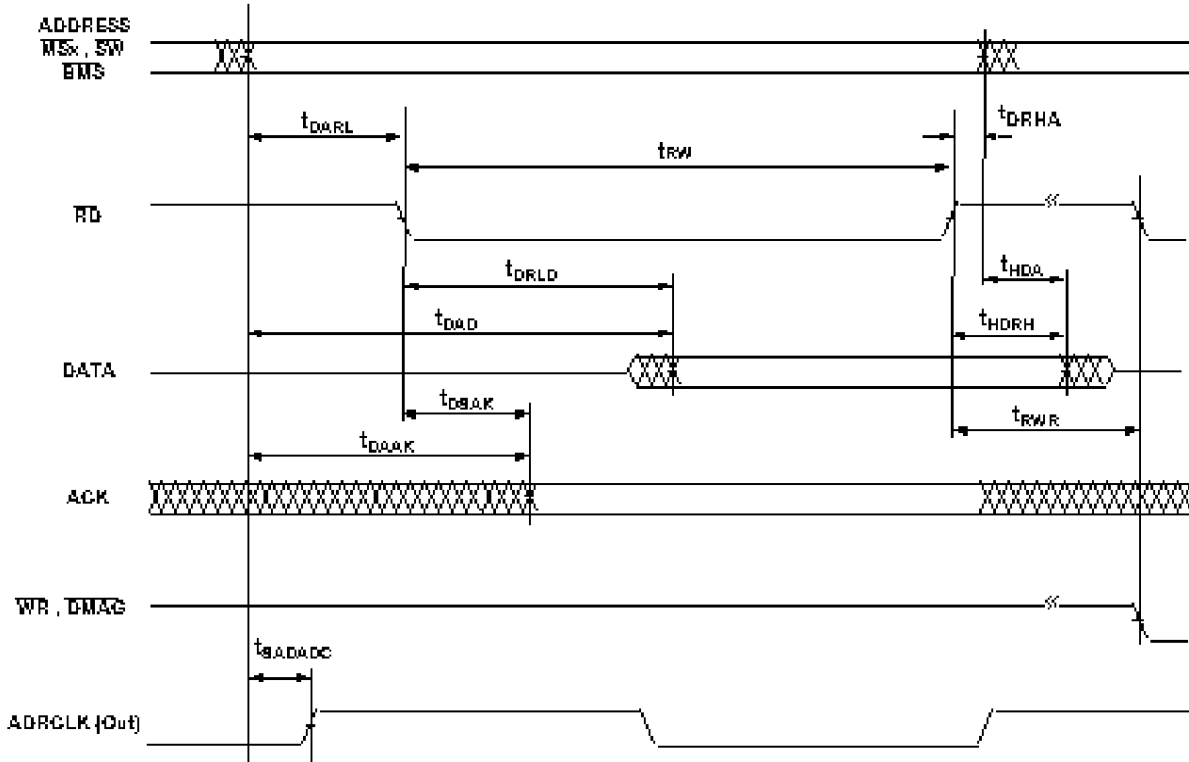
Figure 13 Memory Read - Bus Master
