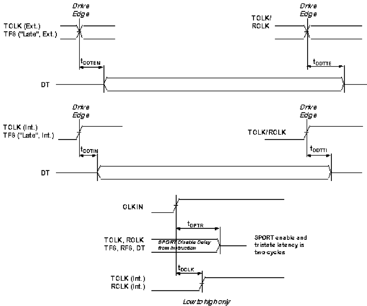
Figure 23 Serial Ports (continued)
