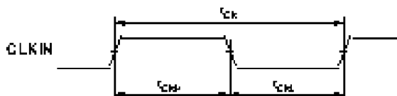
Figure 8 Clock Input
