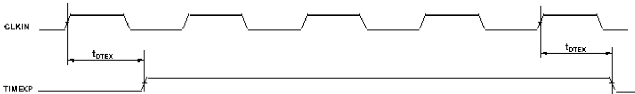
Figure 11 Timer
