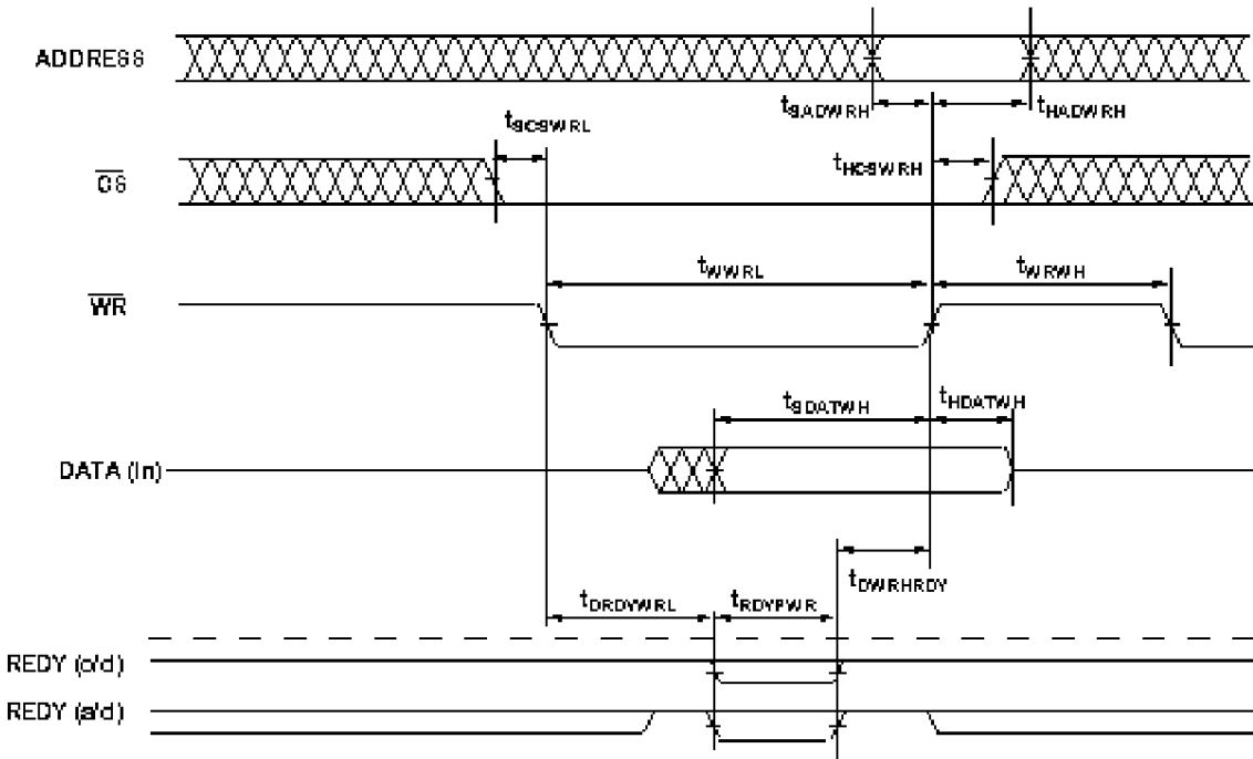
Figure 18 Asynchronous Read/Write -Host to ADSP-21061L
