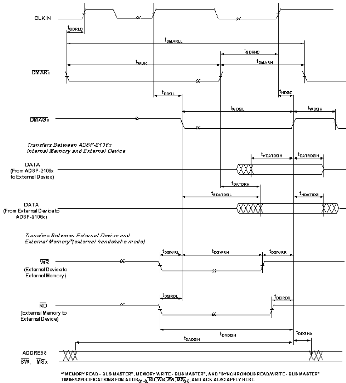
Figure 21 DMA Handshake Timing
