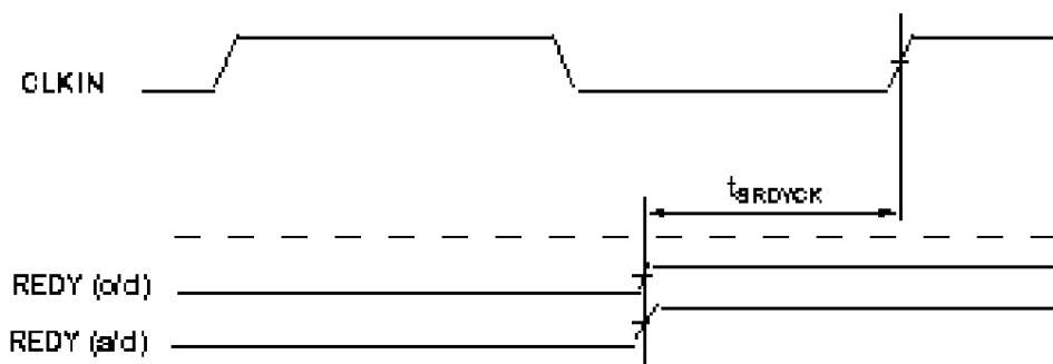
Figure 19 Synchronous REDI Timing
