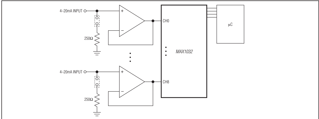
Figure 19. 4–20mA Application
