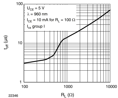
Fig. 3 - Turn-off Time
