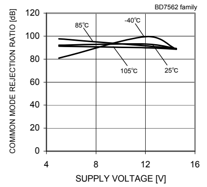
Fig. 41 Common Mode Rejection Ratio – Supply Voltage (VDD=12[V])
