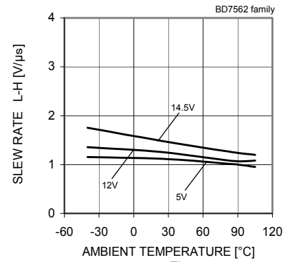
Fig. 44 Slew Rate L-H – Ambient Temperature
