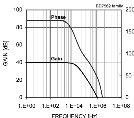
Fig. 46 Gain - Frequency
