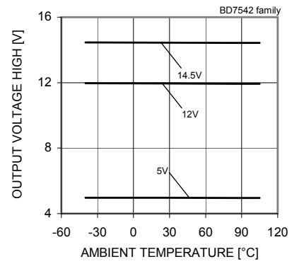
Fig. 75 Output Voltage High - Ambient Temperature ( R_L=10[k\Omega] )
