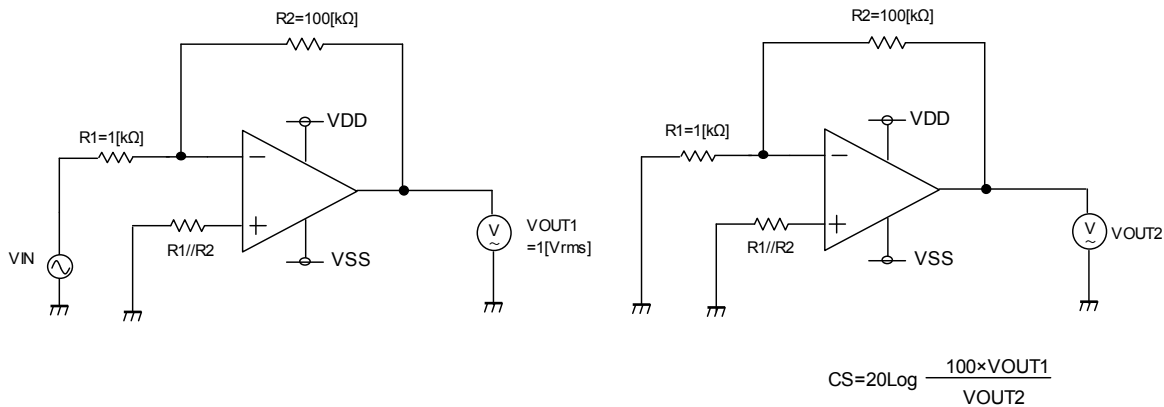
Fig. 97.. Test circuit3
