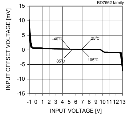
Fig. 38 Input Offset Voltage – Input Voltage (VDD=12[V])
