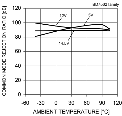
Fig. 42 Common Mode Rejection Ratio – Ambient Temperature (VDD=12[V])
