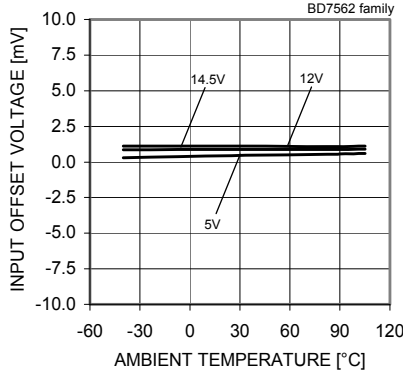
Fig. 37 Input Offset Voltage – Ambient Temperature (Vicm=VDD, VOUT=VDD/2)
