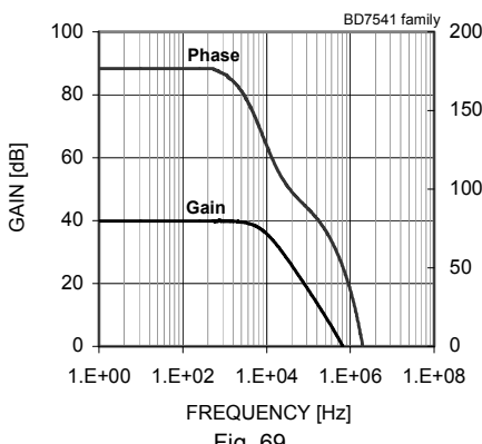
Gain - Frequency
