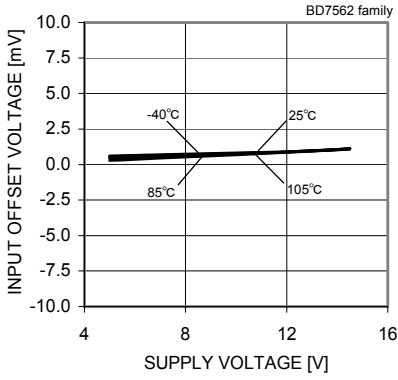
Fig. 36 Input Offset Voltage – Supply Voltage (Vicm=VDD, VOUT=VDD/2)
