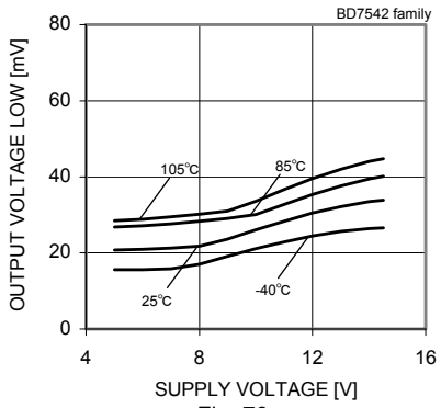
Fig. 76 Output Voltage Low - Supply Voltage ( R_L=10[k\Omega] )
