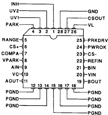
PLCC-28 (Top View)
