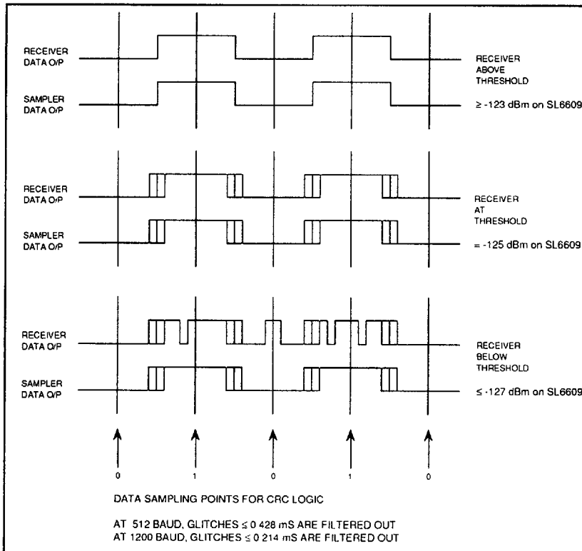
Fig 4 Data Filter Operation
