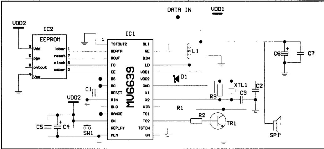
Fig 16 MV6639 Evaluation Circuit
