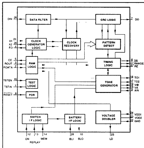
Fig 2 MV6639 Block Diagram
