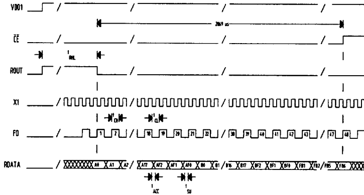
Fig. 7b. Sequence During Refresh or Status Change
