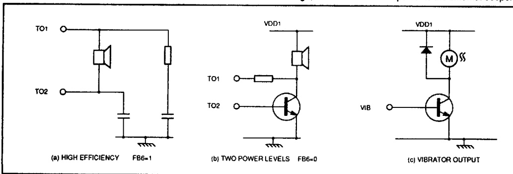
Fig 10 Tone Generator / Vibrator Interface Circuits
