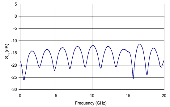
Typical S_{11} Curve
