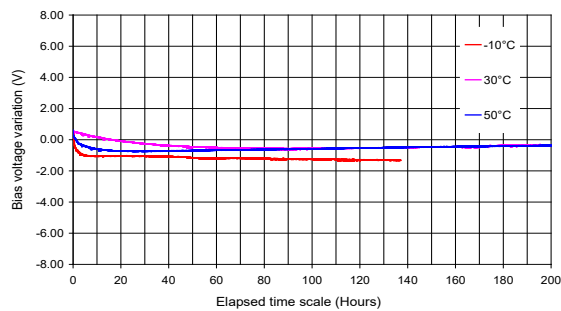
Stability with Time and Temperature
