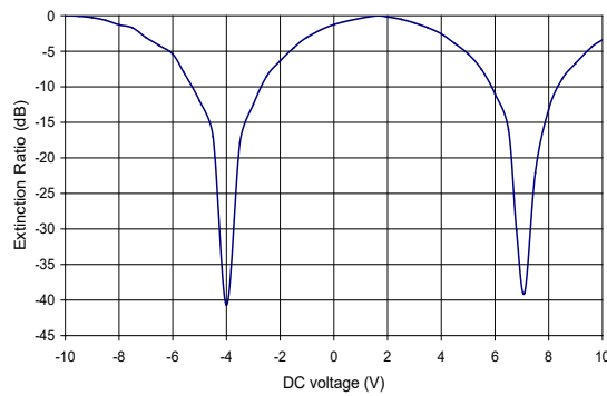
Extinction Ratio
