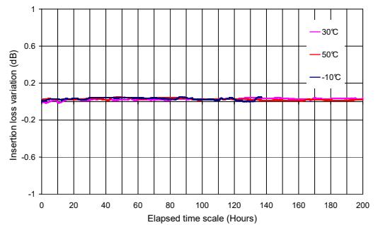
Insertion Loss with Time and Temperature
