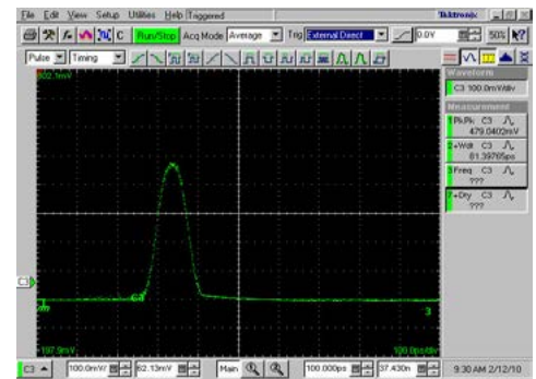
Generated 80 ps Optical Pulse
