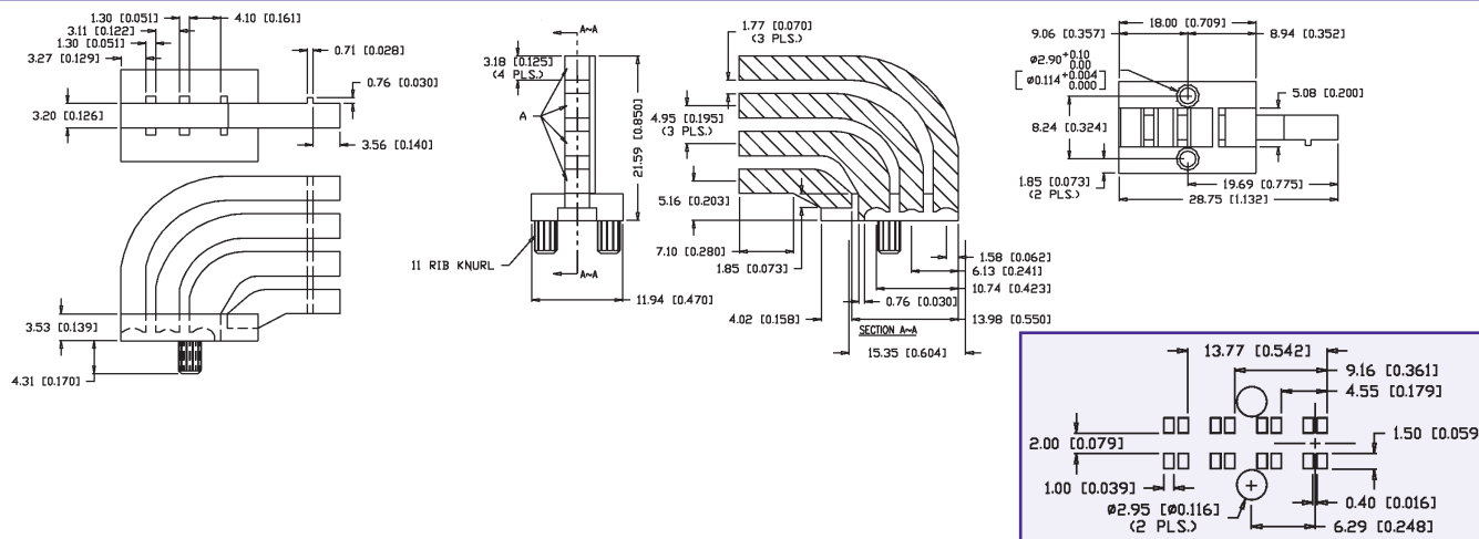
Figure 14 Part # LPF-C041304S
