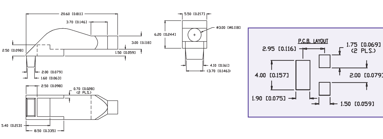
Figure 15 Part # LPF-C011301S
