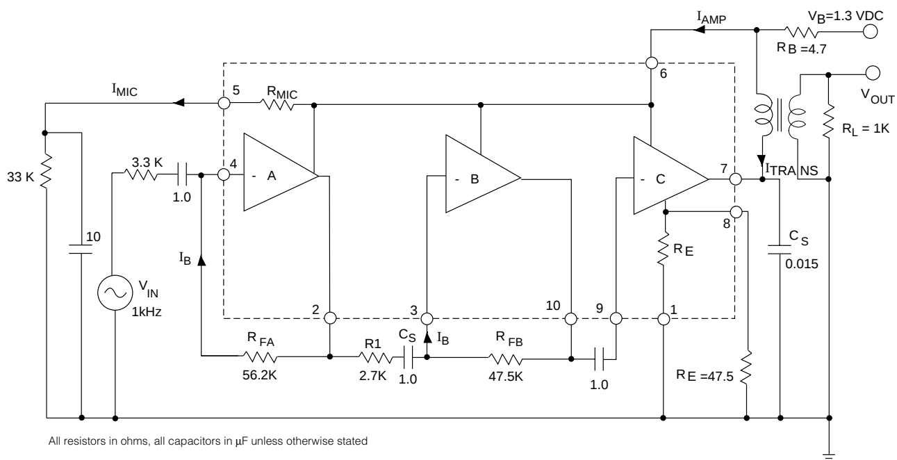
Fig. 1 Test Circuit
