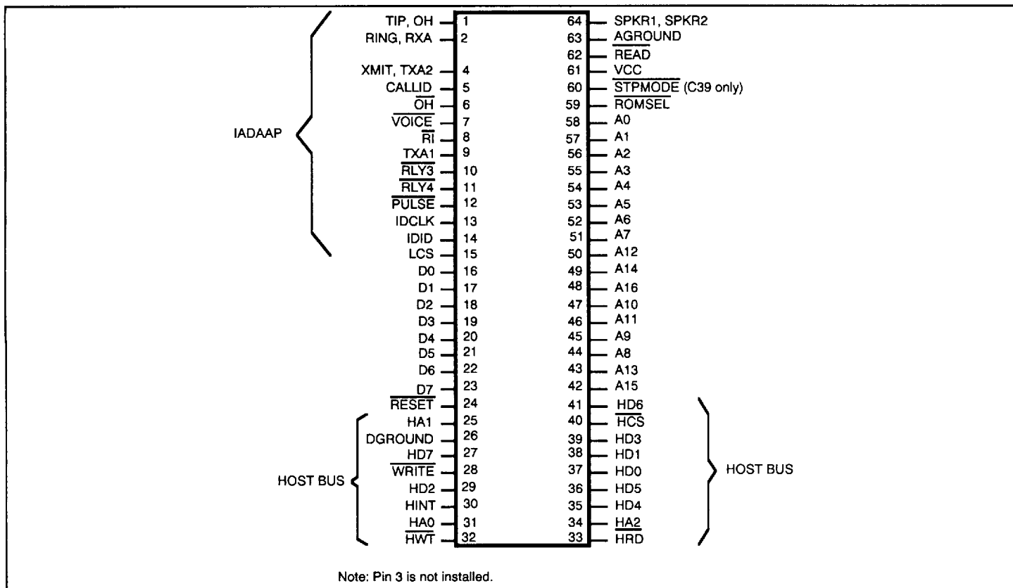
Figure 4. Parallel Pinout
