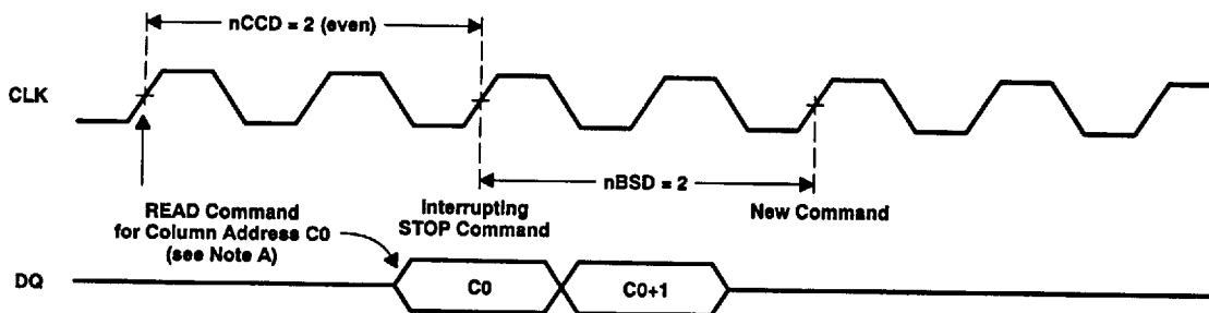
Figure 4. Read Burst Interrupted by STOP Command
