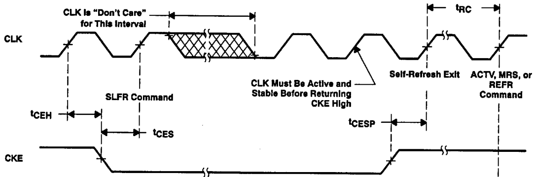
Figure 20. Self-Refresh Entry/Exit
