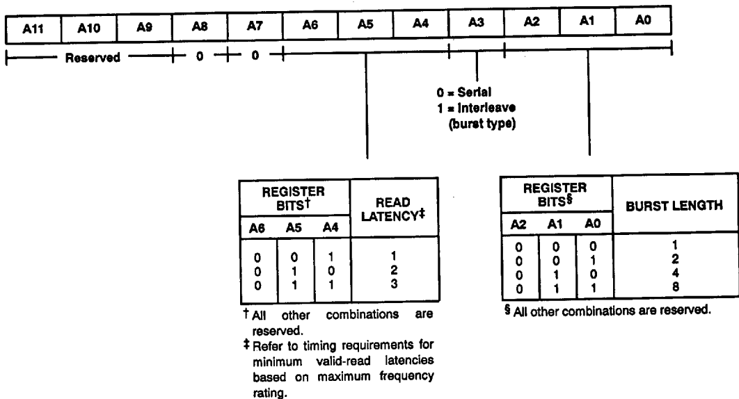
Figure 1. Mode-Register Programming
