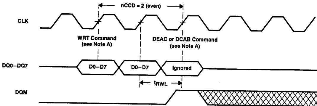
Figure 9. Write Burst Interrupted by DEAC/DCAB Command
