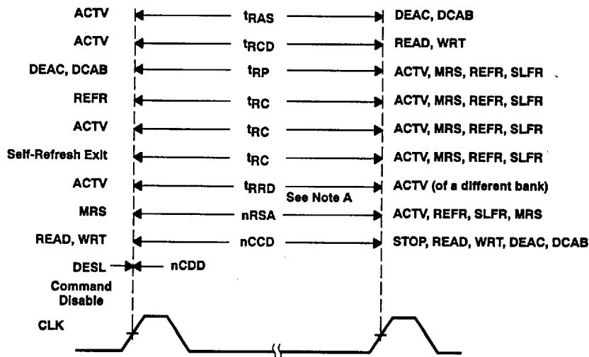
Figure 13. Command-to-Command Parameters
