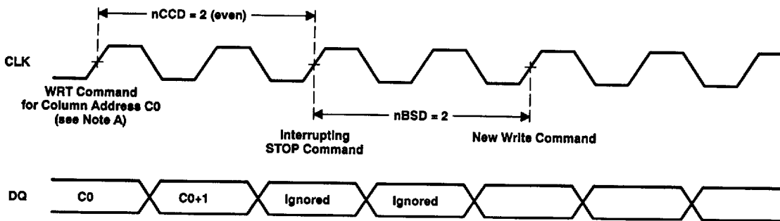
Figure 8. Write Burst Interrupted by STOP Command
