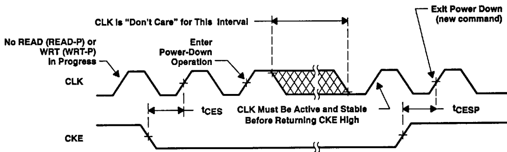
Figure 19. Power-Down Operation
