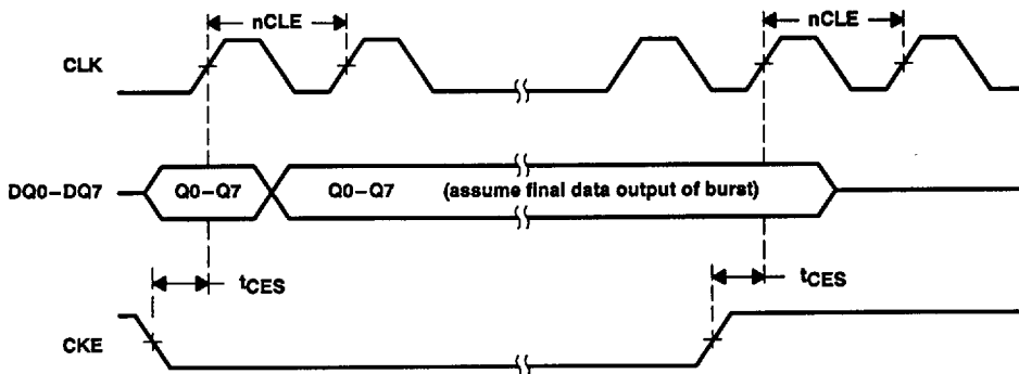
Figure 18. CLK-Suspend Operation
