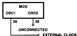
FIGURE 4E. EXTERNAL CLOCK SOURCE CONNECTIONS
