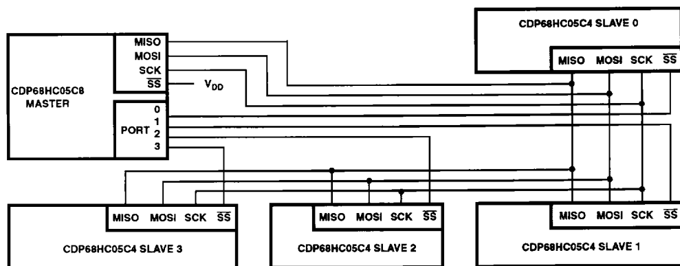
FIGURE 27. MASTER-SLAVE SYSTEM CONFIGURATION (SINGLE MASTER, FOUR SLAVES)
