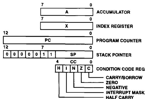
FIGURE 8. PROGRAMMING MODEL
