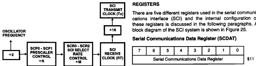
FIGURE 26. RATE GENERATOR DIVISION
