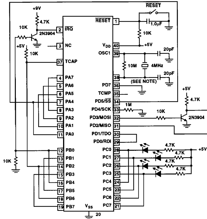
FIGURE 10. SELF-CHECK CIRCUIT SCHEMATIC DIAGRAM
