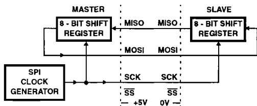
FIGURE 30. SERIAL PRIPHERAL INTERFACE MASTER-SLAVE INTERCONNECTION
