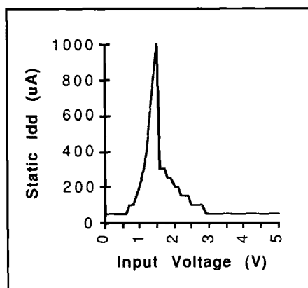
Figure 38: Input Characteristic
