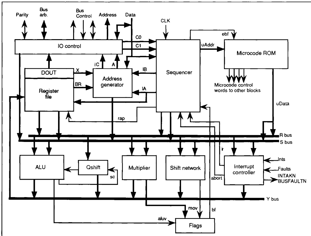
Figure 1: Architecture
