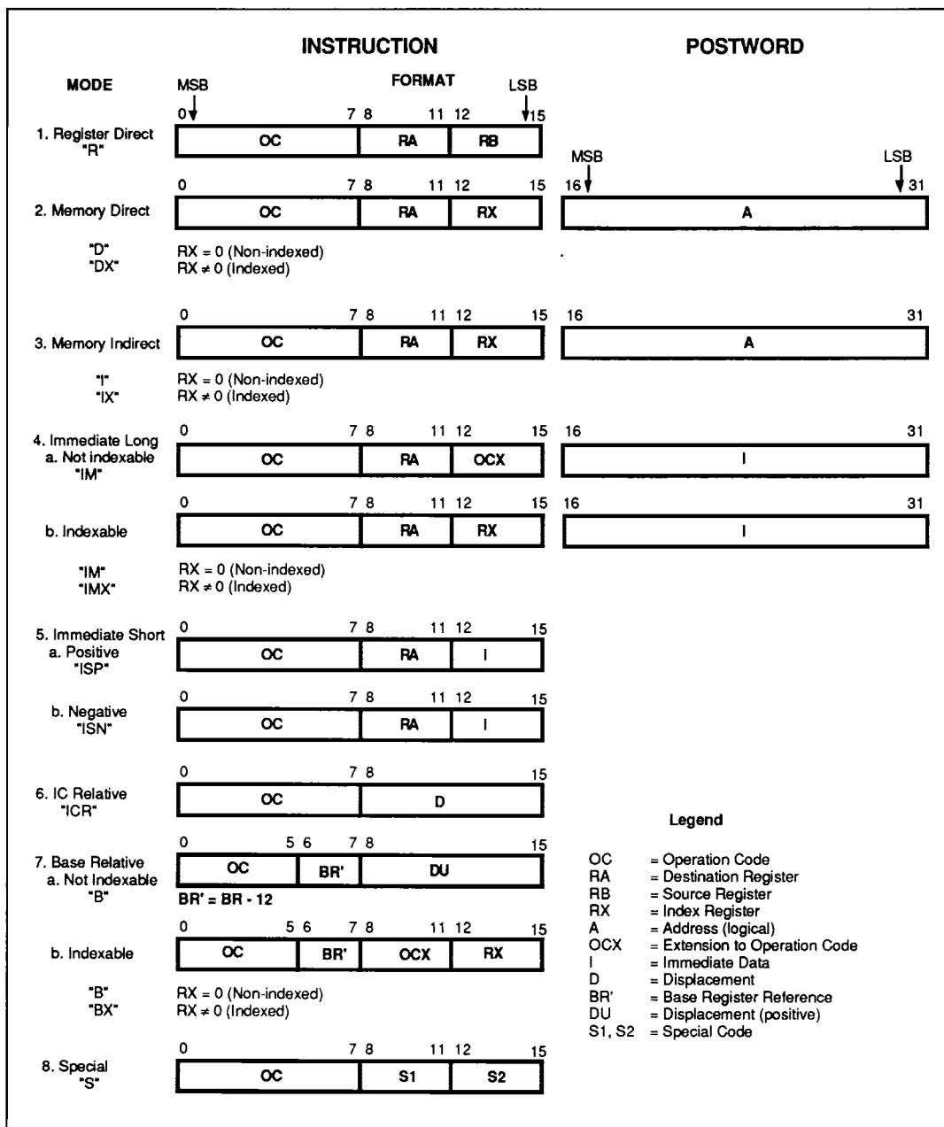
Figure 18: Addressing Modes
