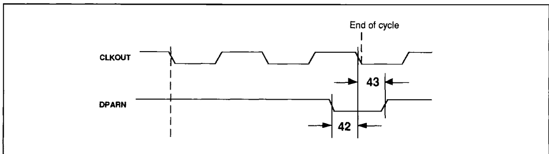
Figure 31: DPARN Timing
