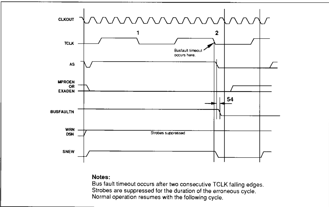
Figure 23b: Bus Fault Timeout
