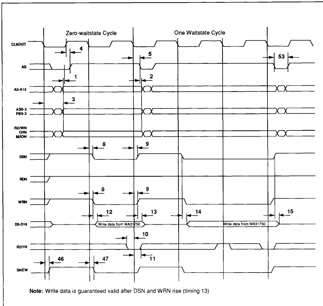
Figure 22: Write Cycle Timings
