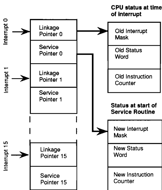
Figure 11: Interrupt Vectoring
