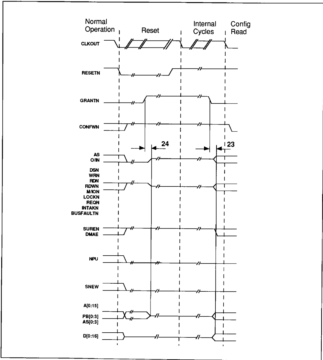
Figure 26: GRANTN during RESETN Low
