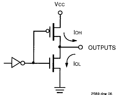
Figure 3. Output Structure
