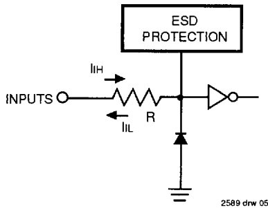
Figure 2. Input Structure
