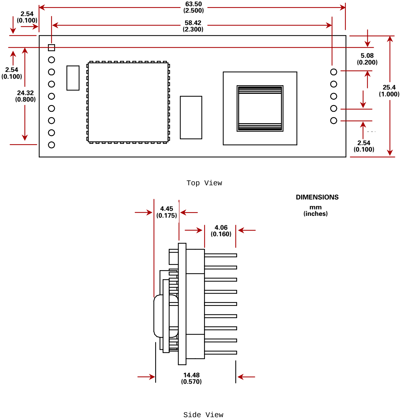
Figure 4. Mechanical Dimensions
