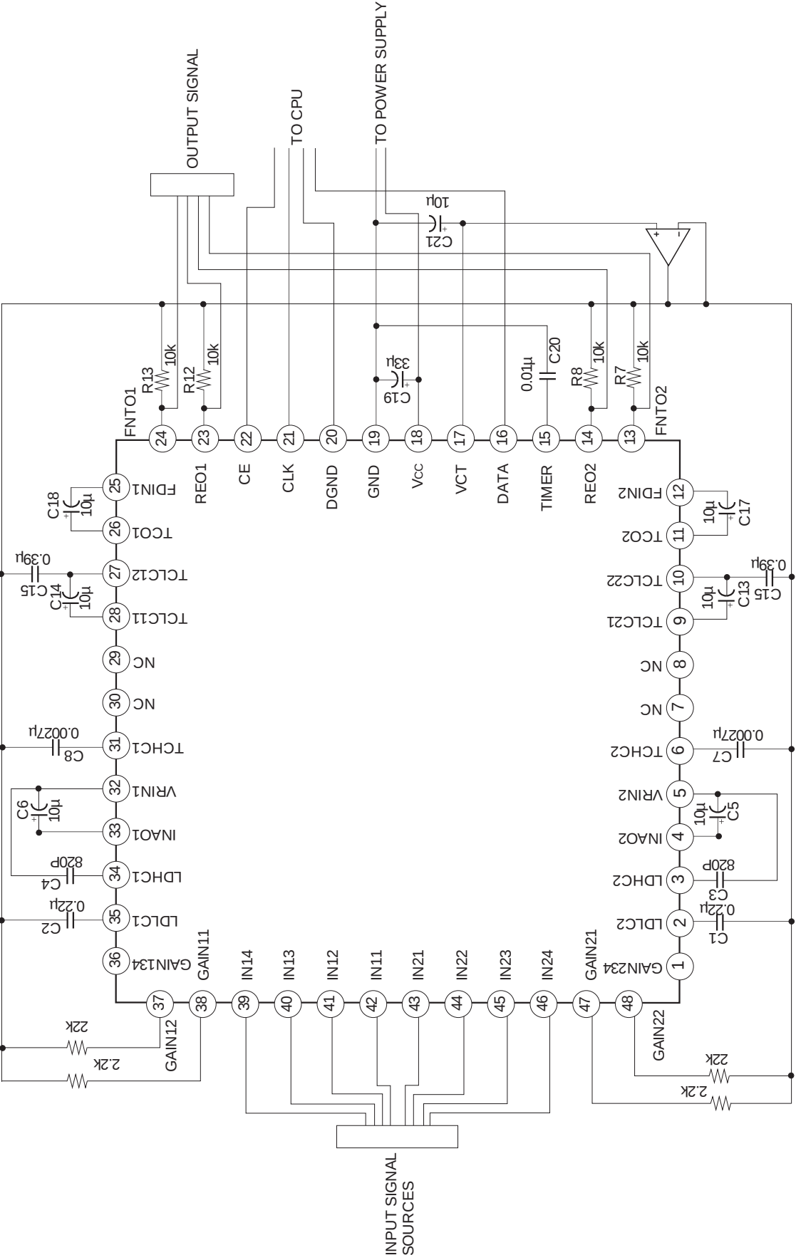
Application Circuit
