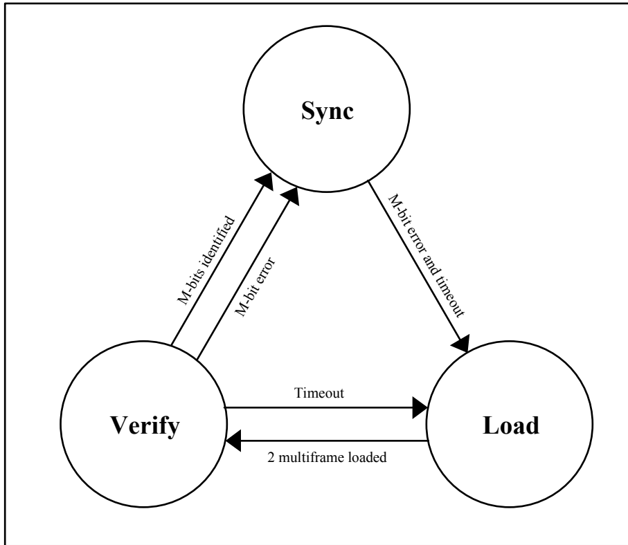
Figure 10-37. DS3 Multiframe Framer State Diagram
