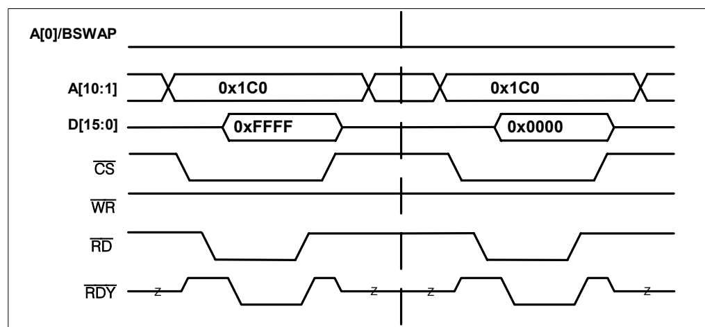
Figure 8-37. Clear Status Latched Register on Read
