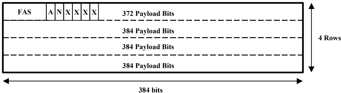
Figure 10-13. Example E3 G.751 Internal Fractional Frame
