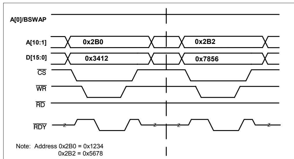
Figure 8-36. 16-Bit Mode with Byte Swap
