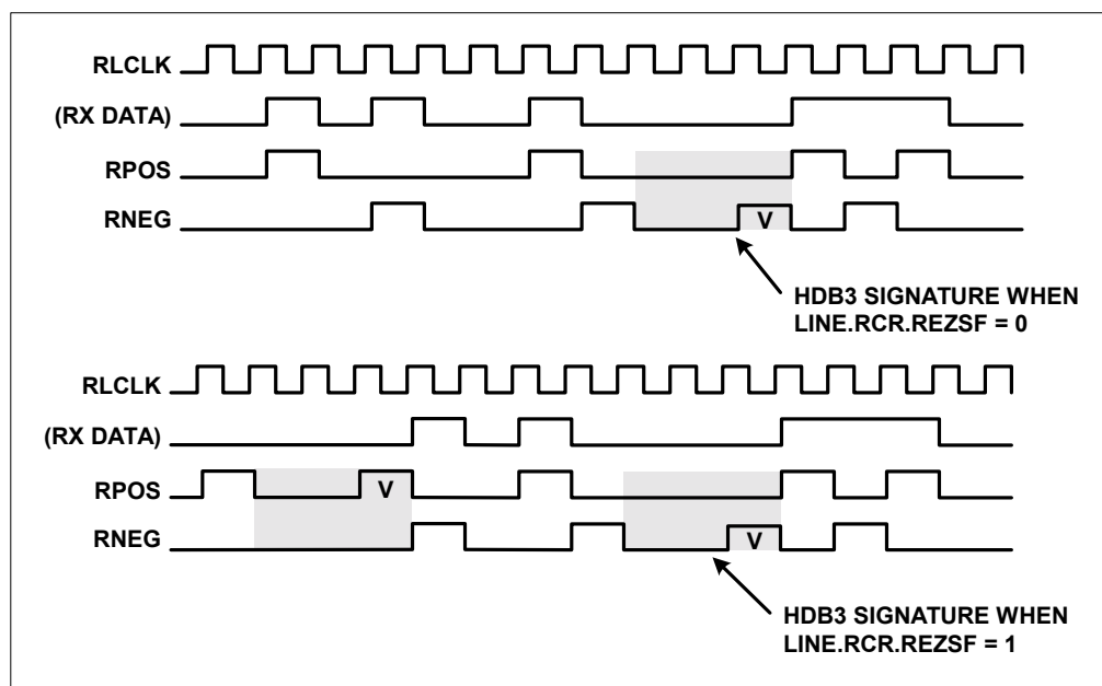
Figure 10-48. HDB3 Signatures
