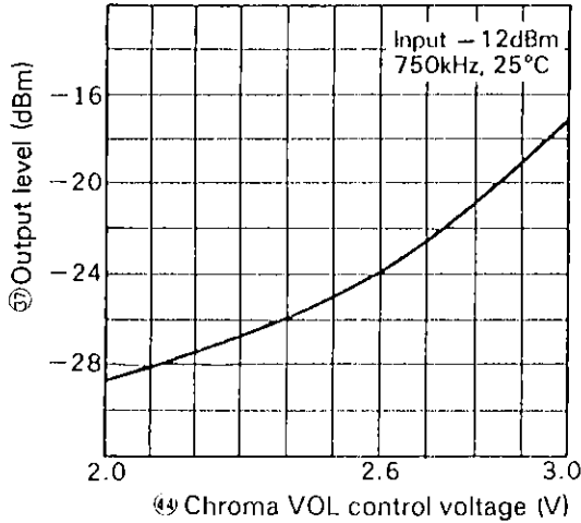
Output level vs. Chroma VOL control voltage
