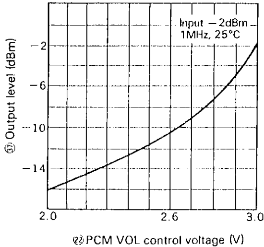
Output level vs. PCM VOL control voltage
