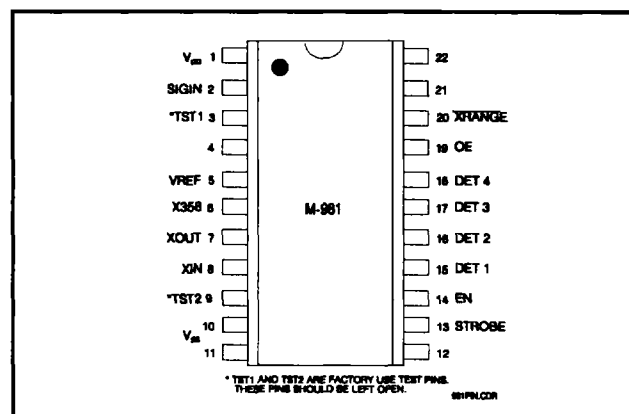
Figure 1 Pin Diagram
