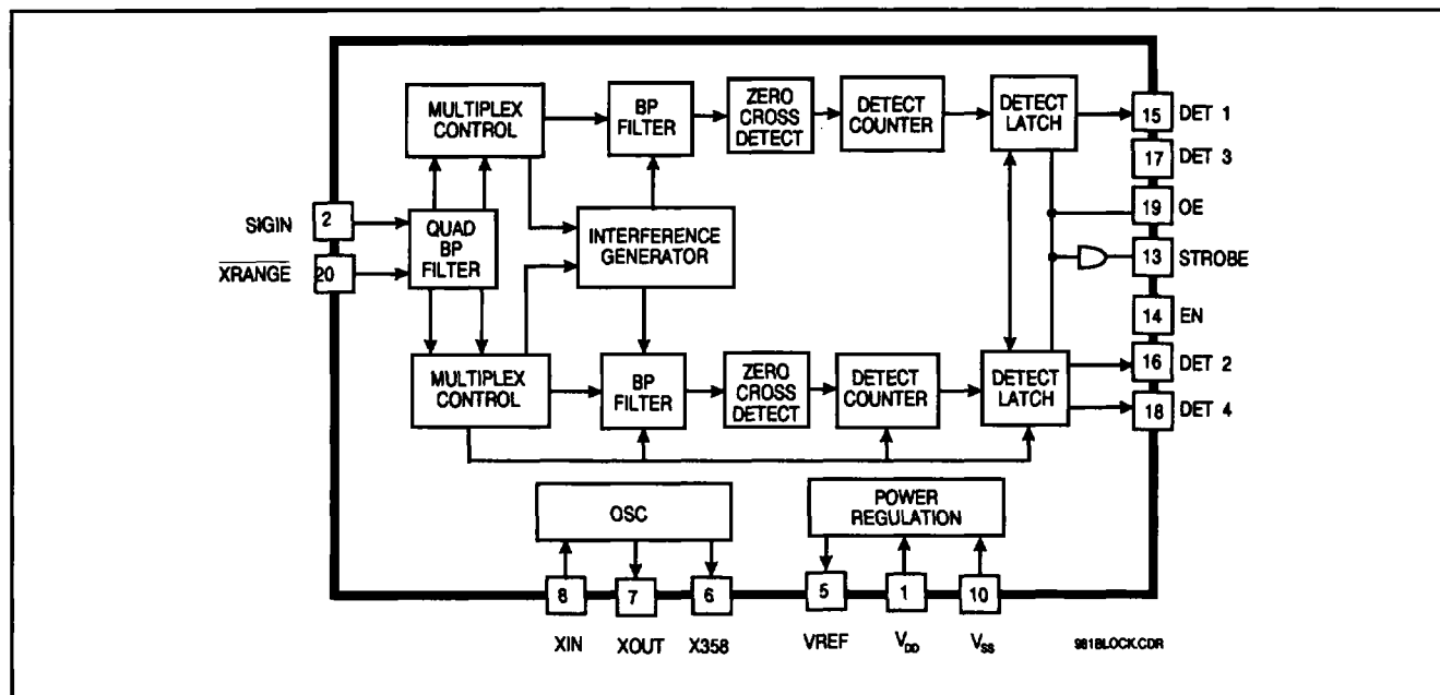
Figure 2 Block Diagram
