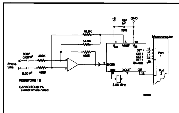
Figure 4 A Telephone Line Circuit Application
