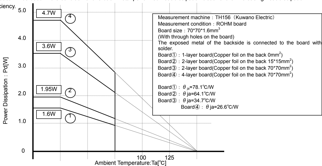
Fig.2 HTSSOP-B40 Derating Curve
