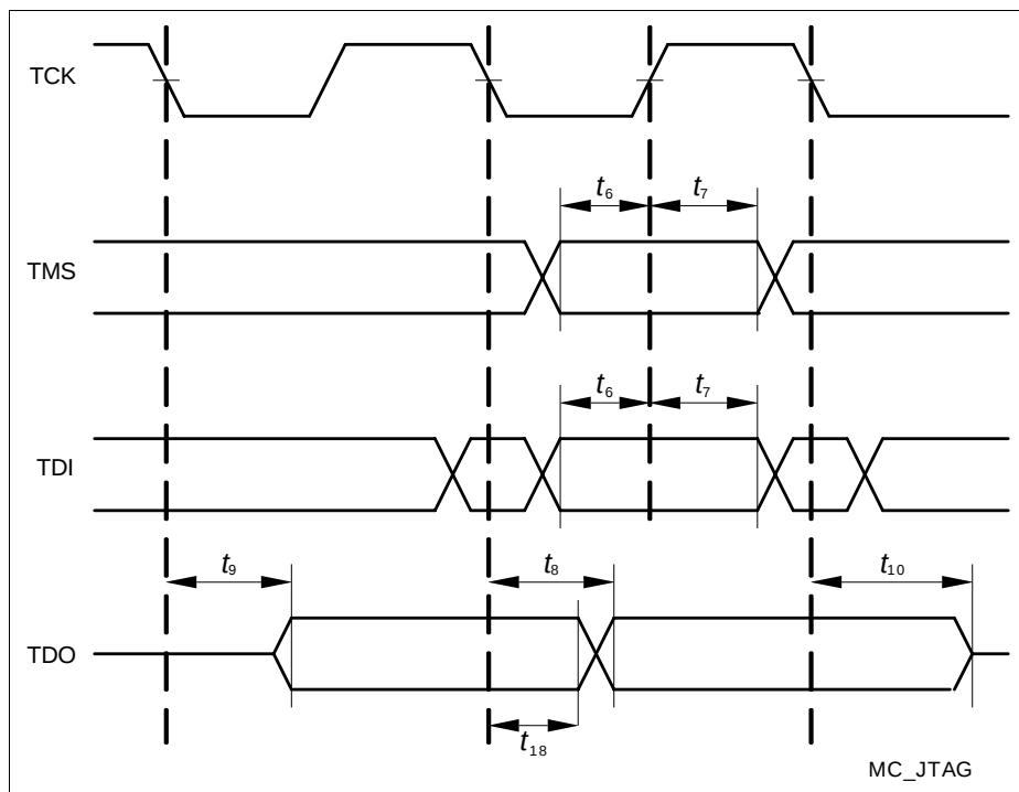
Figure 32 JTAG Timing
