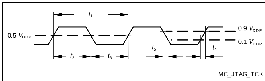
Figure 31 Test Clock Timing (TCK)
