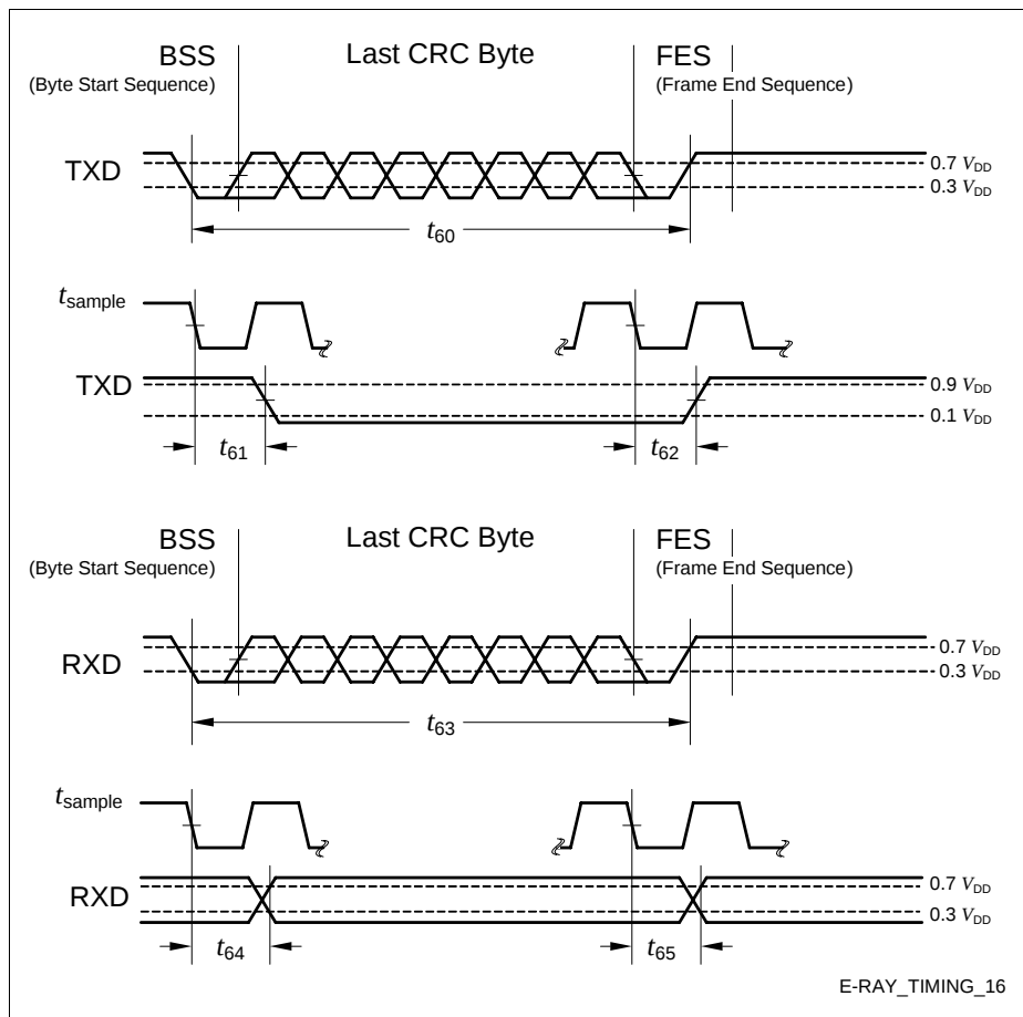
Figure 27 FlexRay Timing
