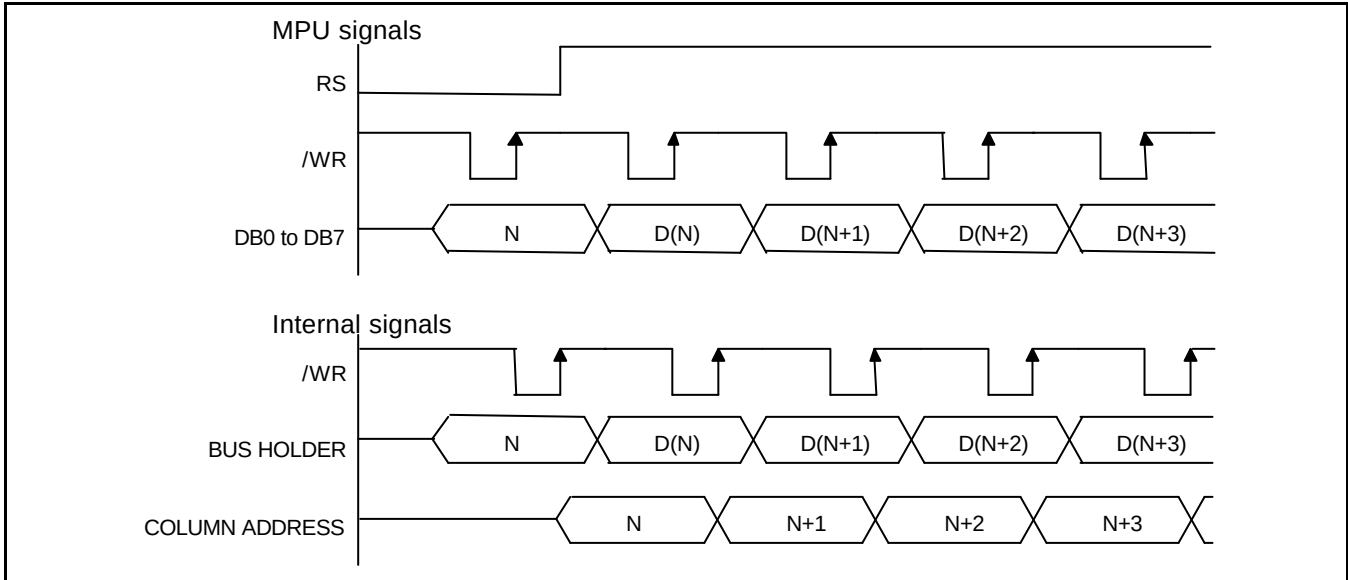
Figure 8. Write Timing
