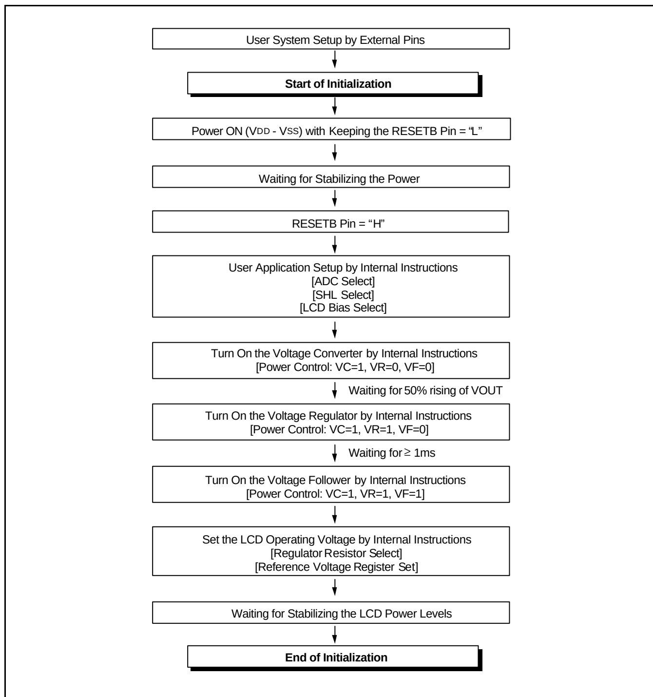
Figure 31. Initializing with the Built-in Power Supply Circuits
