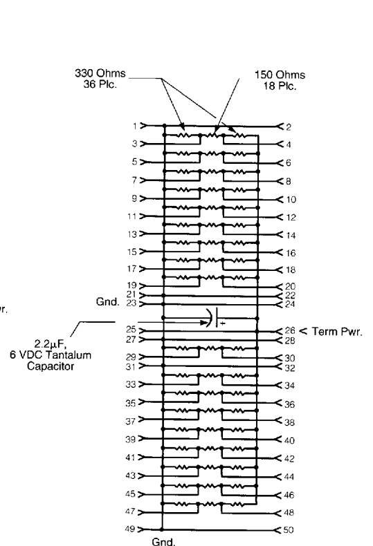
50-Position, Differential, with Capacitor Part No. 869362-1
