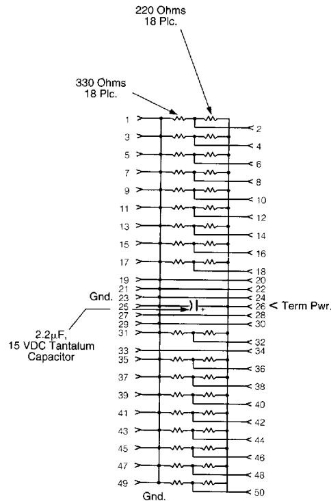
50-Position, Single-Ended, with Capacitor Part No. 869333-1
